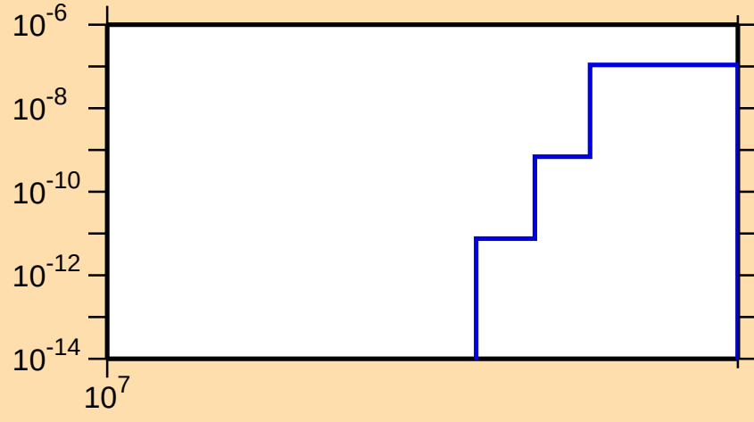
\sigma vs. E for ^{158}\text{Lu}(n,nt)
