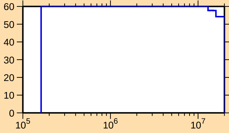
\Delta\sigma/\sigma vs. E for ^{158}\text{Lu}(n,n\text{cont.})
