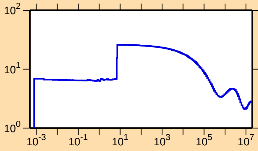
\sigma vs. E for ^{158}\text{Lu}(n,\text{el.})
