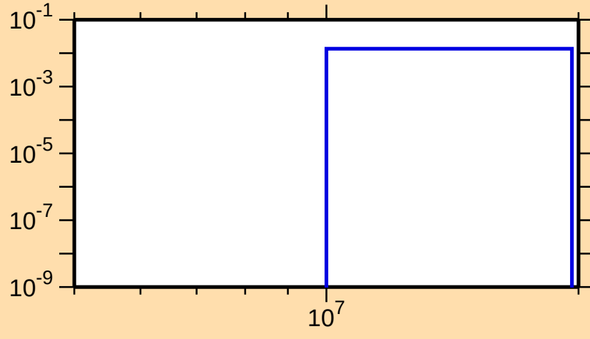
\sigma vs. E for ^{158}\text{Lu}(n,2np)
