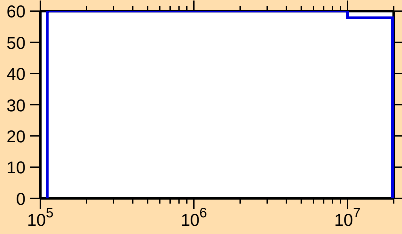
\Delta\sigma/\sigma vs. E for ^{158}\text{Lu}(n,\text{inel.})
