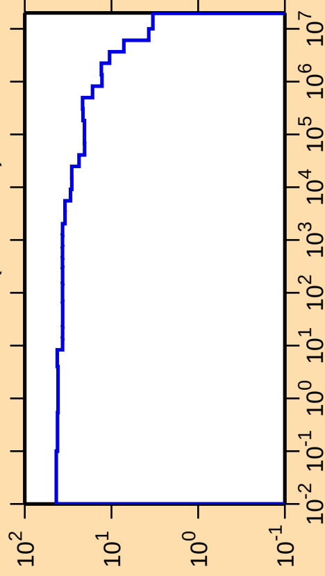
\Delta\sigma/\sigma vs. E for ^{158}\text{Lu}(n,\text{nonel.})
