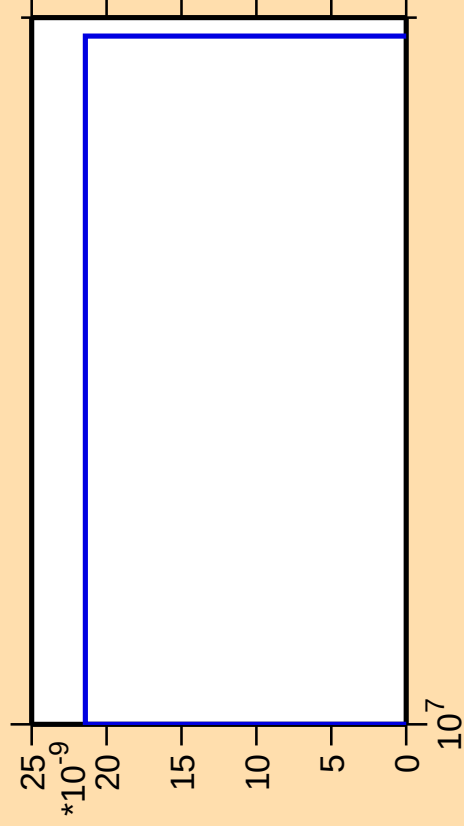
\Delta\sigma/\sigma vs. E for ^{158}\text{Lu}(\text{mt 11})
