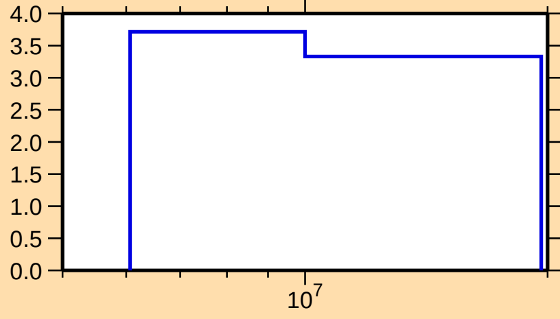
\Delta\sigma/\sigma vs. E for ^{158}\text{Lu}(n,\text{nonel.})
