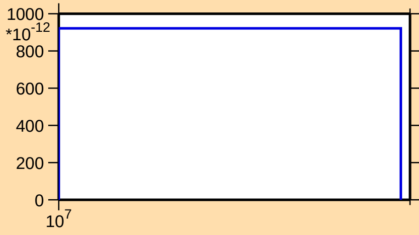
\sigma vs. E for ^{158}\text{Lu}(n,nt)
