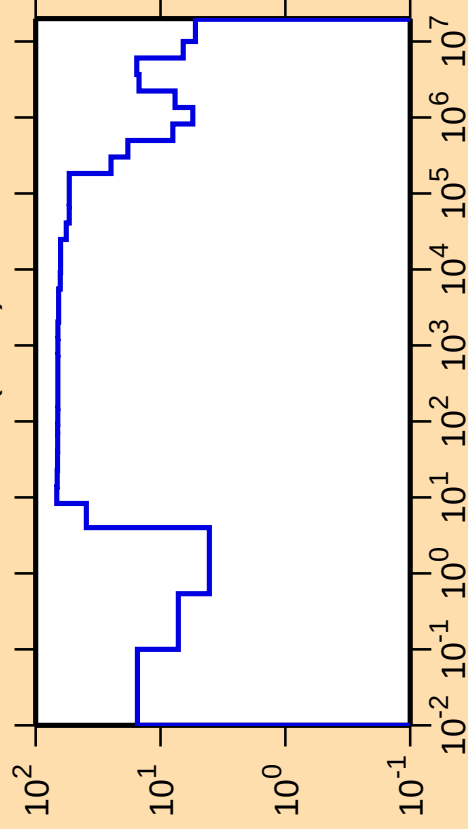
\Delta\sigma/\sigma vs. E for ^{158}\text{Lu}(n,\text{el.})
