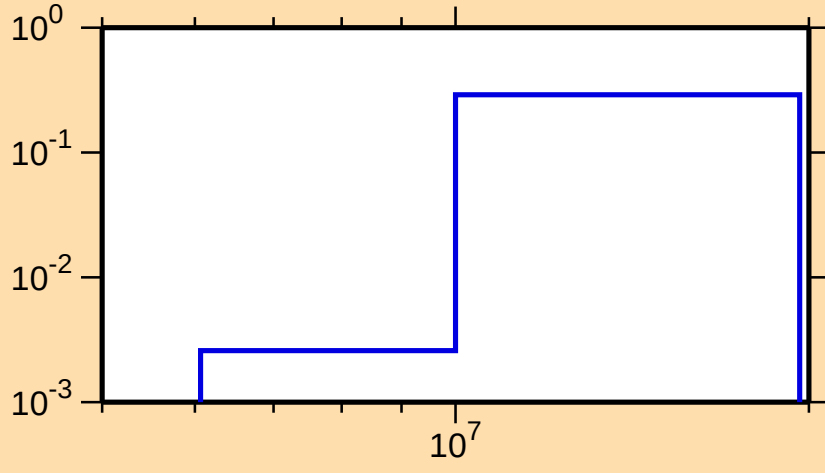
\sigma vs. E for ^{158}\text{Lu}(n,2n)
