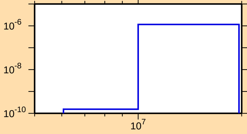
\sigma vs. E for ^{158}\text{Lu}(\text{mt117})
