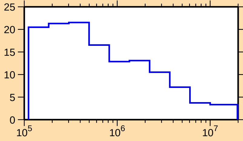
\Delta\sigma/\sigma vs. E for ^{158}\text{Lu}(n,\text{nonel.})
