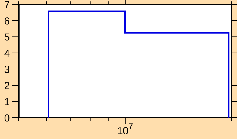
\Delta\sigma/\sigma vs. E for ^{158}\text{Lu}(n,\text{el.})
