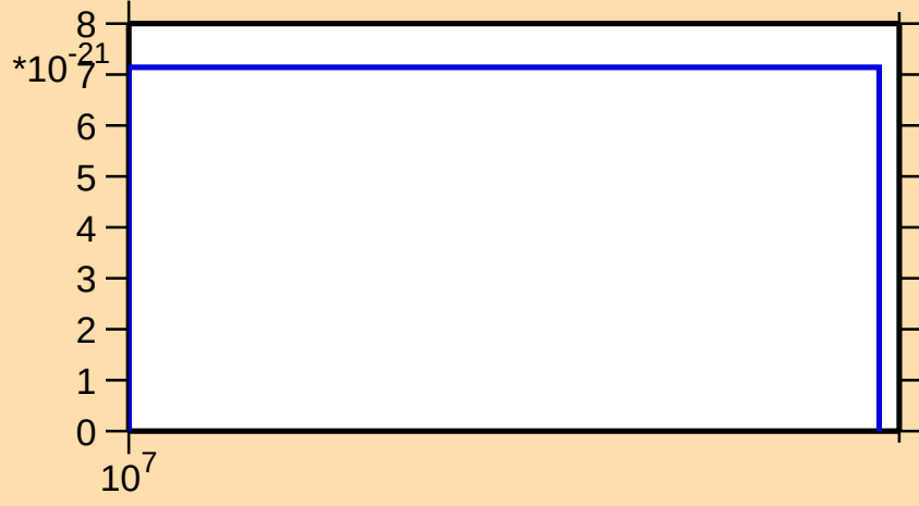
\sigma vs. E for ^{158}\text{Lu}(\text{mt 11})
