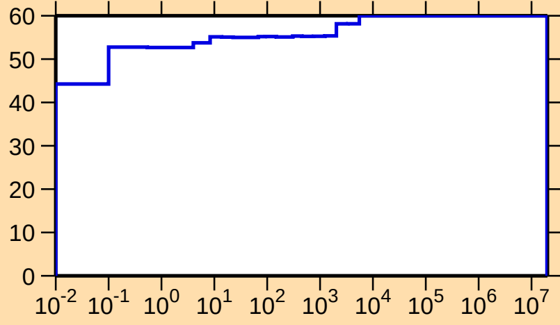
\Delta\sigma/\sigma vs. E for ^{158}\text{Lu}(n,p)
