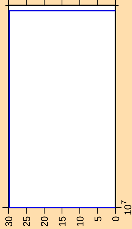
\Delta\sigma/\sigma vs. E for ^{158}\text{Lu}(n,3n\alpha)
