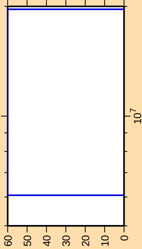
\Delta\sigma/\sigma vs. E for ^{158}\text{Lu}(\text{mt117})
