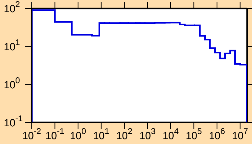
\Delta\sigma/\sigma vs. E for ^{158}\text{Lu}(n,\text{tot.})
