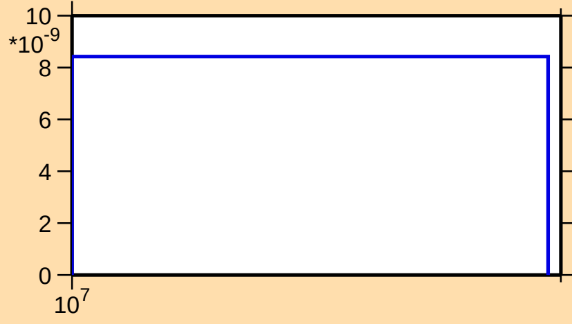
\sigma vs. E for ^{158}\text{Lu}(n,3n\alpha)
