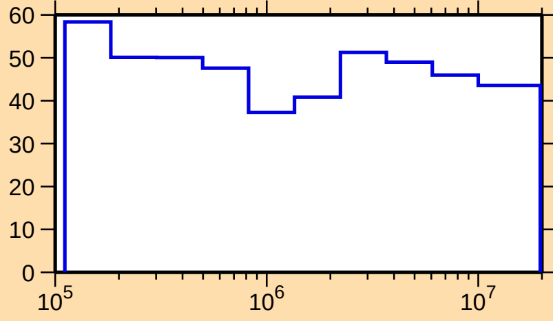
\Delta\sigma/\sigma vs. E for ^{158}\text{Lu}(n,n_1)
