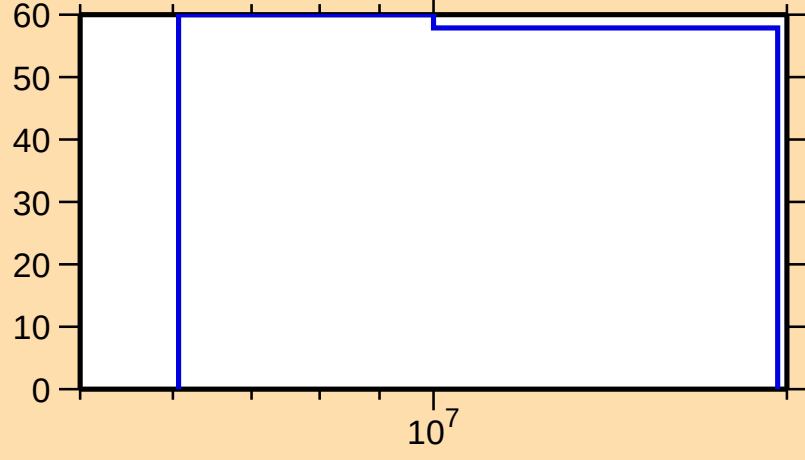
\Delta\sigma/\sigma vs. E for ^{158}\text{Lu}(n,\text{inel.})
