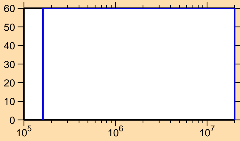
\Delta\sigma/\sigma vs. E for ^{159}\text{Lu}(n,n_1)
