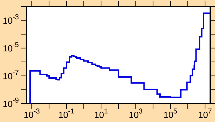
\sigma vs. E for ^{159}\text{Lu}(n,p\alpha)
