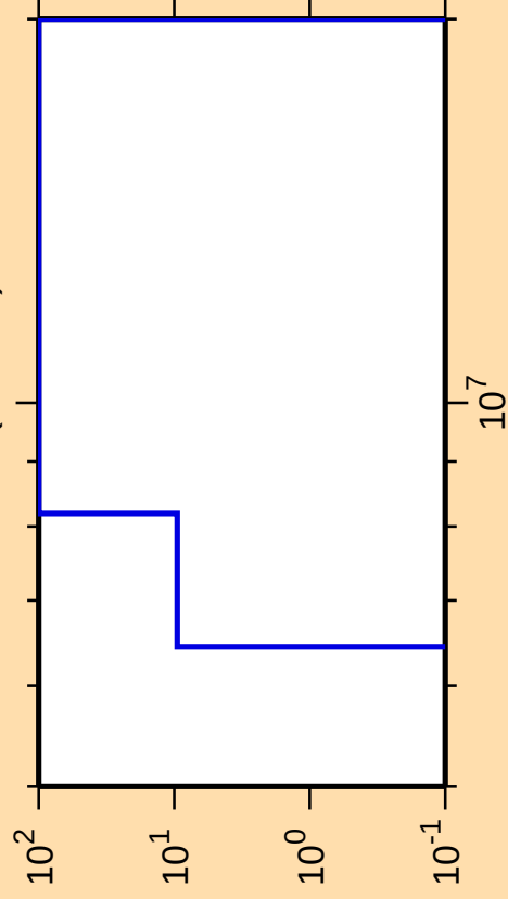
\Delta\sigma/\sigma vs. E for ^{159}\text{Lu}(\text{mt117})
