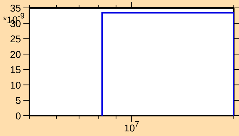
\sigma vs. E for ^{159}\text{Lu}(n,3n)
