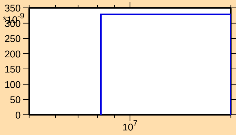
\sigma vs. E for ^{159}\text{Lu}(n,\text{pd})
