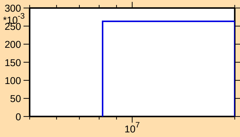
\sigma vs. E for ^{159}\text{Lu}(n,2n)
