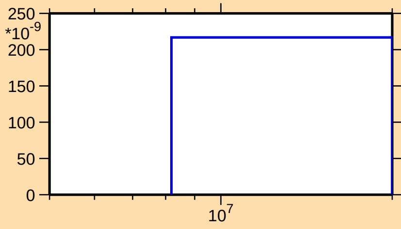
\sigma vs. E for ^{159}\text{Lu}(n,\text{nd})
