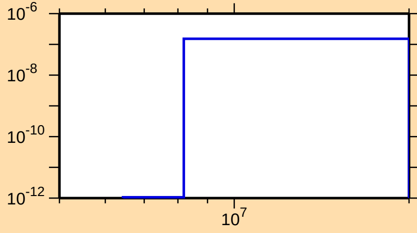
\sigma vs. E for ^{159}\text{Lu}(\text{mt117})
