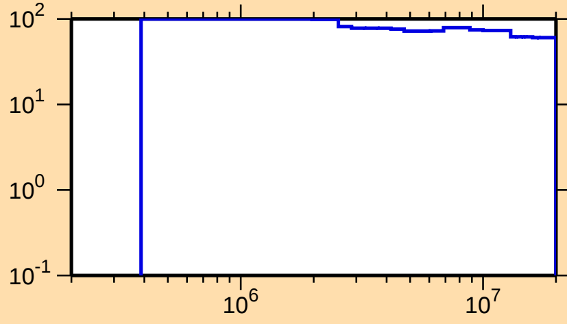
\Delta\sigma/\sigma vs. E for ^{160}\text{Lu}(n,n\text{cont.})
