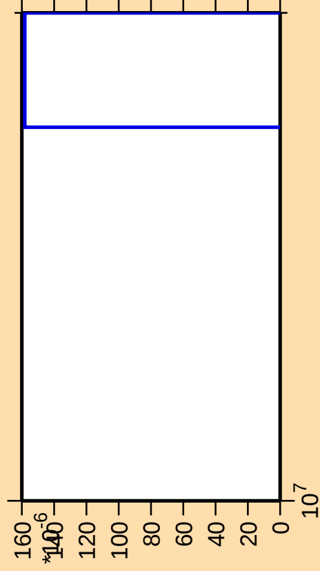
\Delta\sigma/\sigma vs. E for ^{160}\text{Lu} (mt 11)
