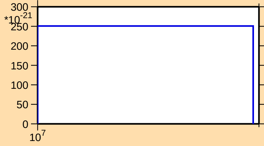
\sigma vs. E for ^{160}\text{Lu} (mt 11)
