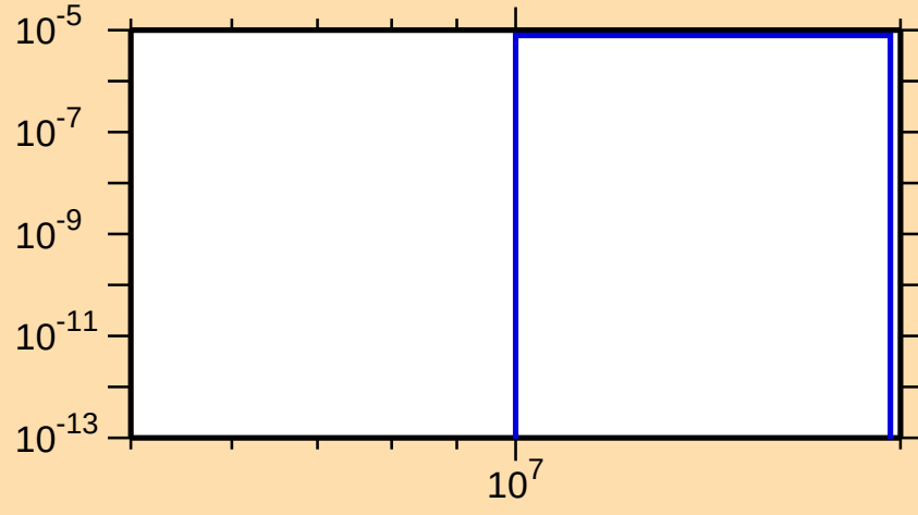
\sigma vs. E for ^{160}\text{Lu}(n,\text{nd})
