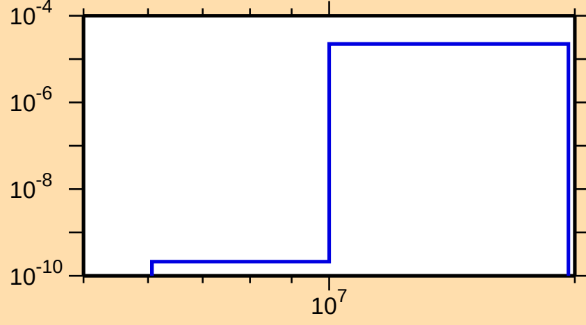
\sigma vs. E for ^{160}\text{Lu}(\text{mt } 45)
