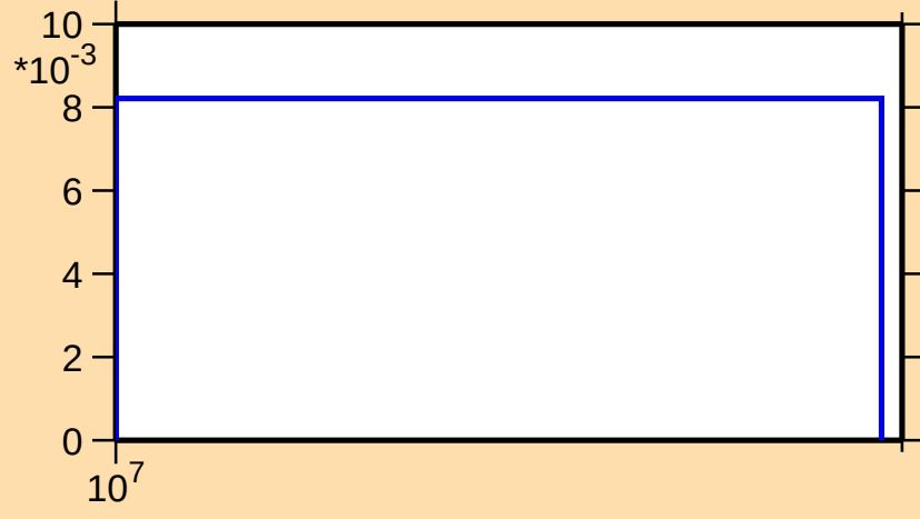
\sigma vs. E for ^{160}\text{Lu}(n,2np)
