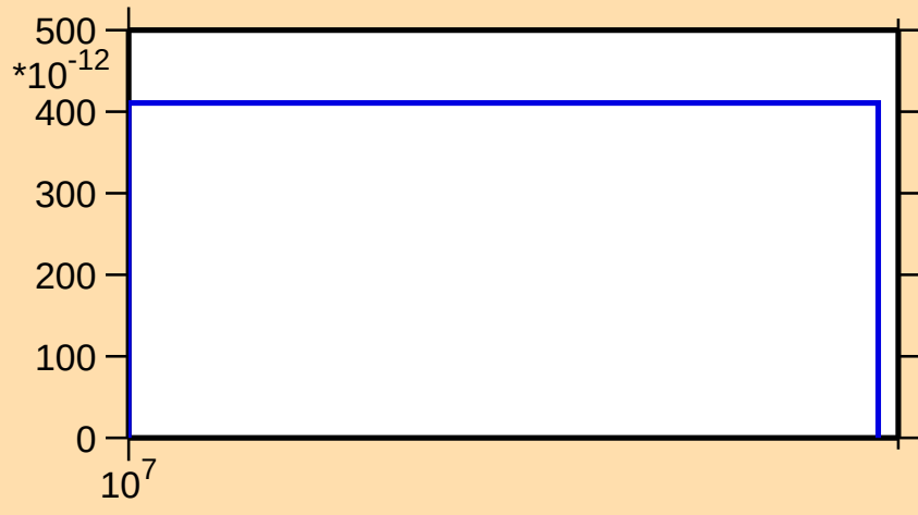
\sigma vs. E for ^{160}\text{Lu}(n,\text{nt})
