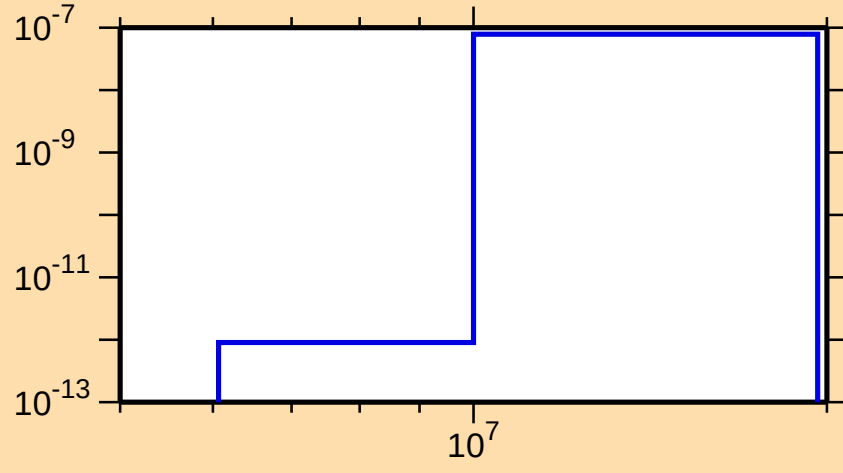
\sigma vs. E for ^{160}\text{Lu}(\text{mt117})
