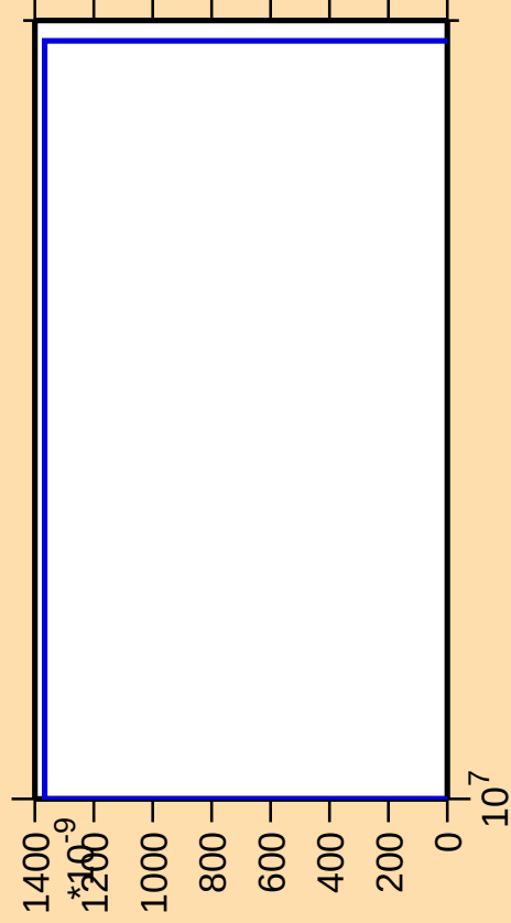
\Delta\sigma/\sigma vs. E for ^{160}\text{Lu} (mt 11)
