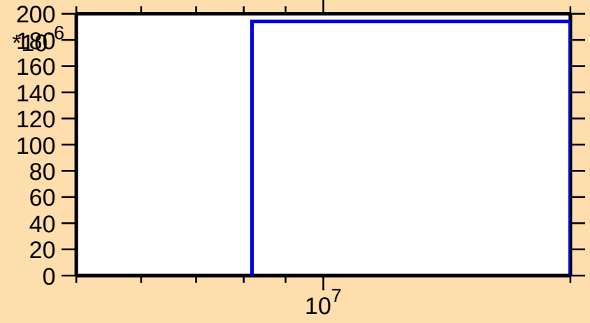
\sigma vs. E for ^{160}\text{Lu}(n,2n\alpha)
