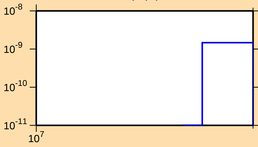
\sigma vs. E for ^{161}\text{Lu}(n,\text{pt})
