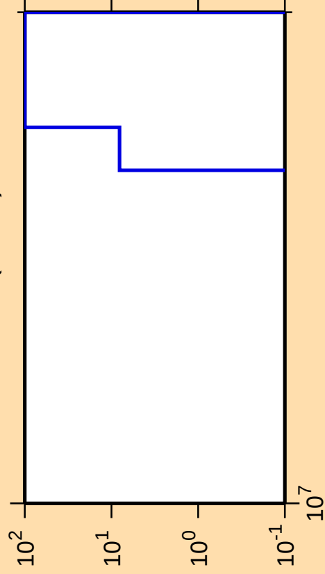
\Delta\sigma/\sigma vs. E for ^{161}\text{Lu} (mt 34)
