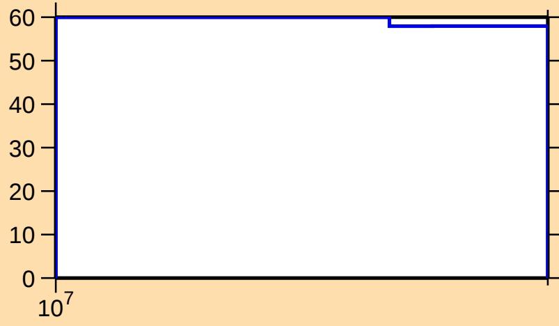
\Delta\sigma/\sigma vs. E for ^{161}\text{Lu}(n,\text{inel.})
