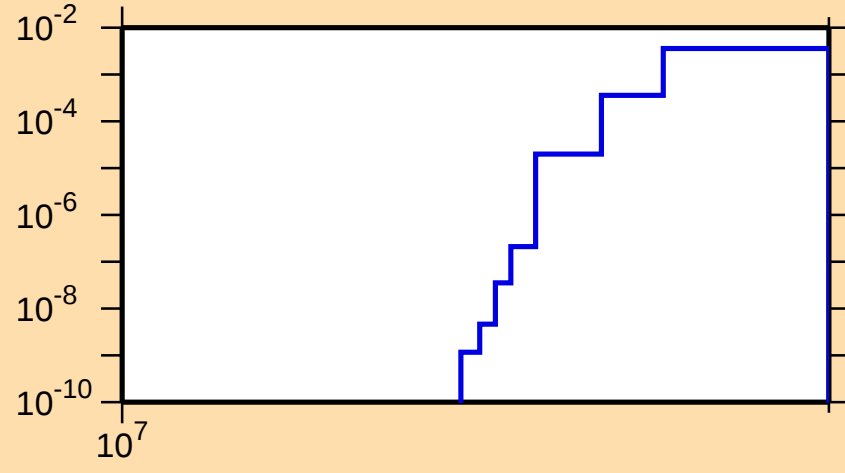
\sigma vs. E for ^{161}\text{Lu}(n,2np)
