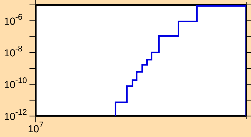
\sigma vs. E for ^{161}\text{Lu}(n,\text{nd})
