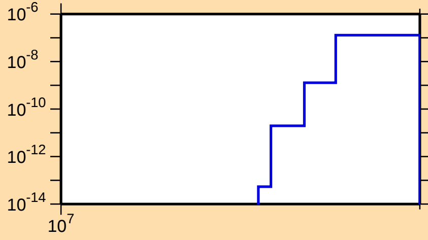
\sigma vs. E for ^{161}\text{Lu}(n,nt)
