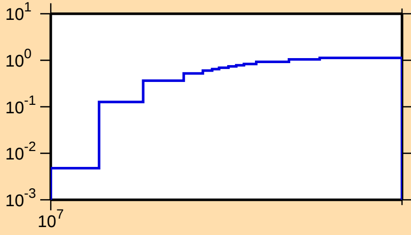
\sigma vs. E for ^{161}\text{Lu}(n,2n)
