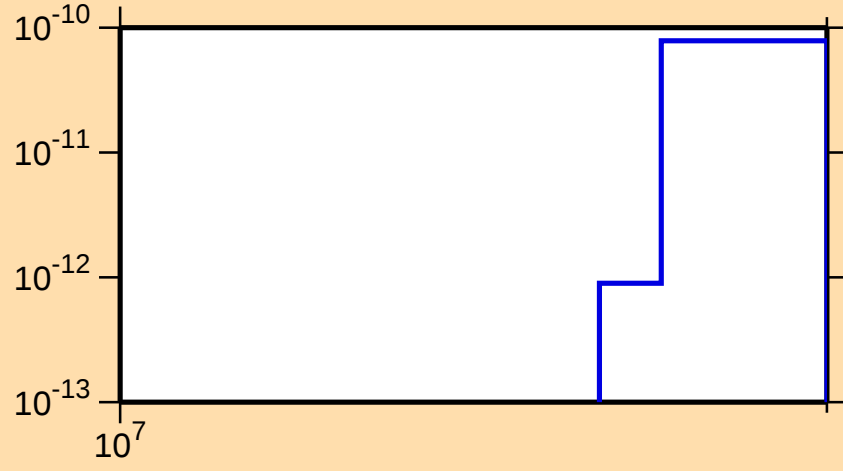
\sigma vs. E for ^{161}\text{Lu} (mt 34)
