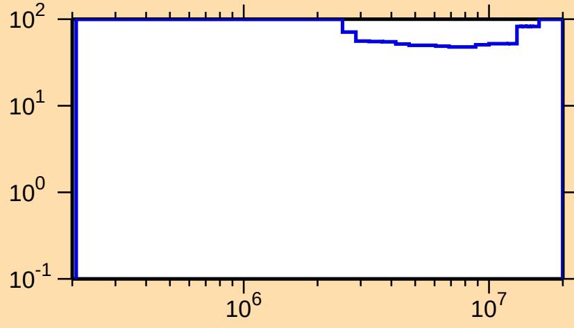
\Delta\sigma/\sigma vs. E for ^{162}\text{Lu}(n,\text{ncont.})
