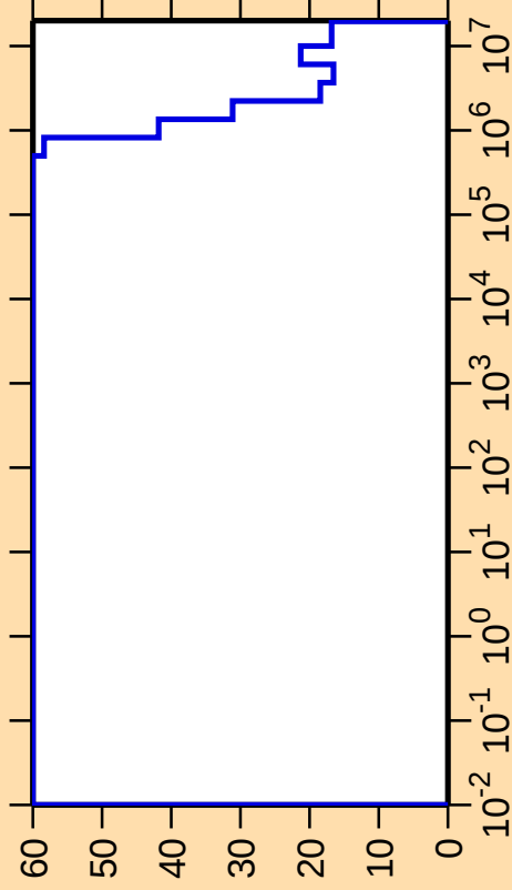
\Delta\sigma/\sigma vs. E for ^{162}\text{Lu}(n,\text{nonel.})
