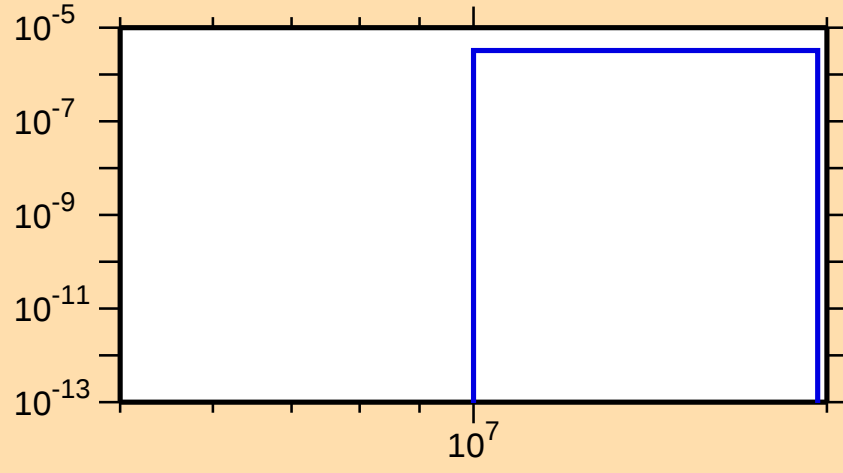
\sigma vs. E for ^{162}\text{Lu}(n,\text{nd})
