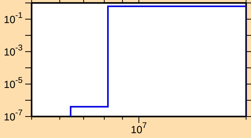
\sigma vs. E for ^{162}\text{Lu}(n,2n)
