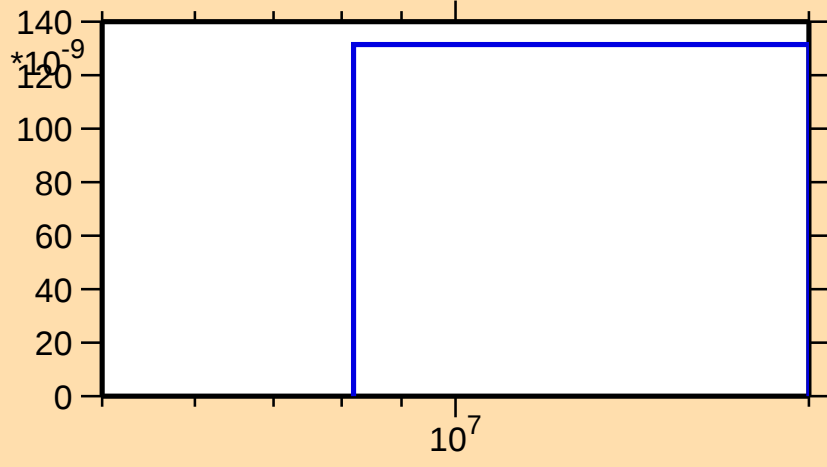
\sigma vs. E for ^{162}\text{Lu} (mt 45)
