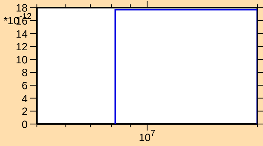
\sigma vs. E for ^{162}\text{Lu}(\text{mt } 34)
