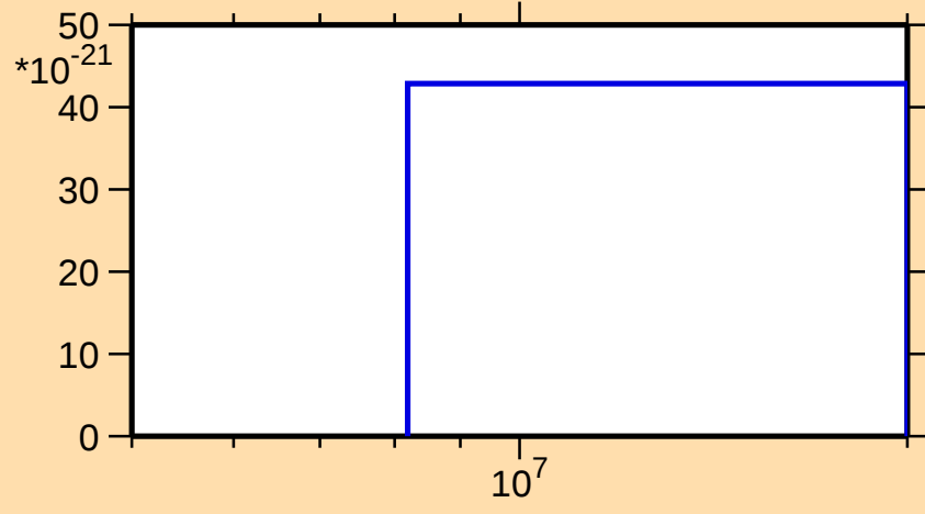
\sigma vs. E for ^{162}\text{Lu}(\text{mt } 11)
