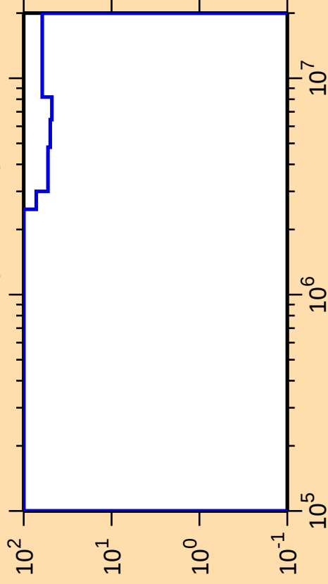
\Delta\sigma/\sigma vs. E for ^{162}\text{Lu}(n,\text{ncont.})
