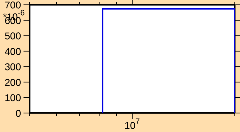
\sigma vs. E for ^{162}\text{Lu}(n,2np)
