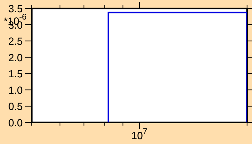
\sigma vs. E for ^{162}\text{Lu}(n,2n\alpha)
