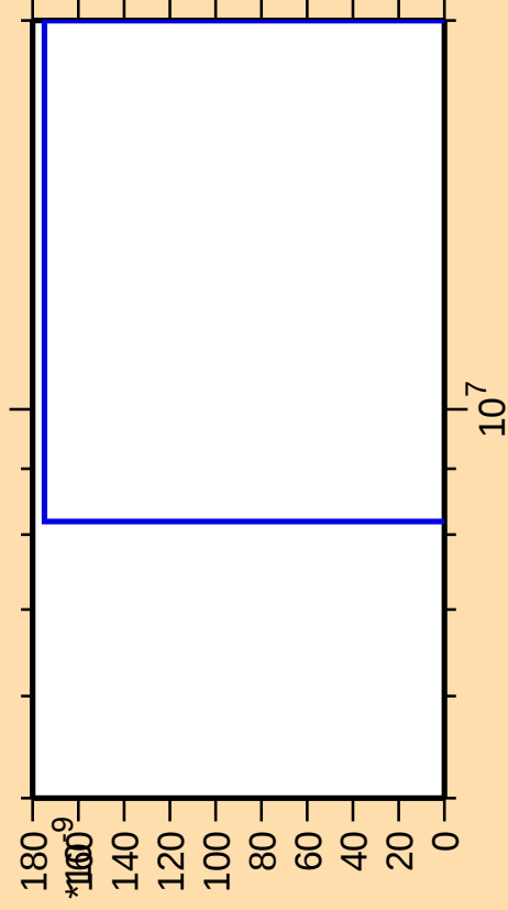
\Delta\sigma/\sigma vs. E for ^{162}\text{Lu}(\text{mt } 11)
