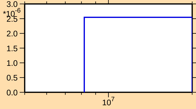
\sigma vs. E for ^{162}\text{Lu}(n,\text{nd})
