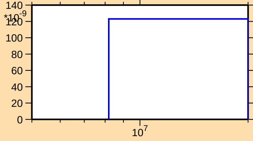
\sigma vs. E for ^{162}\text{Lu} (mt 45)
