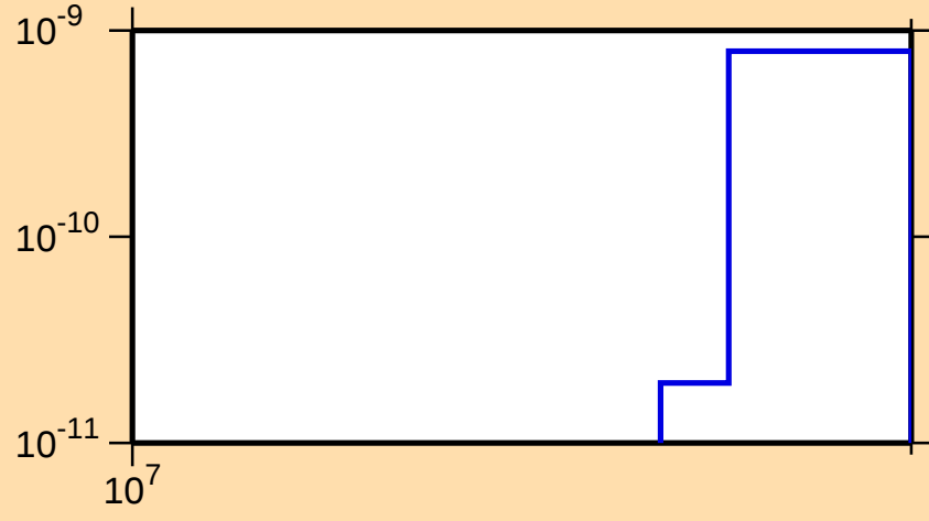
\sigma vs. E for ^{164}\text{Lu} (mt 34)
