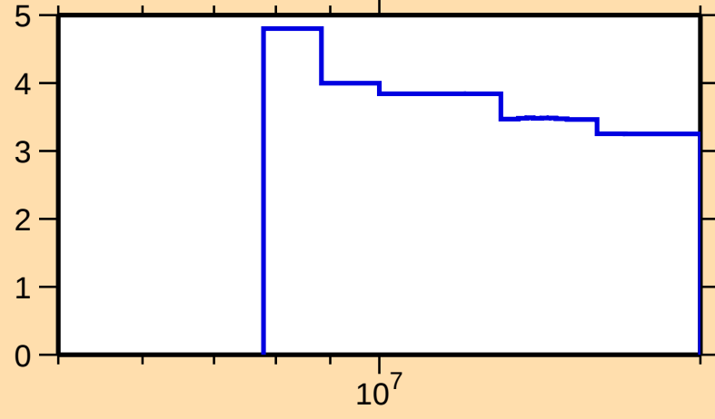
\Delta\sigma/\sigma vs. E for ^{164}\text{Lu}(n,\text{nonel.})
