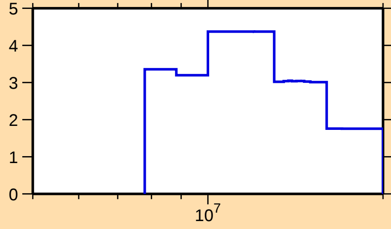
\Delta\sigma/\sigma vs. E for ^{164}\text{Lu}(n,\text{tot.})
