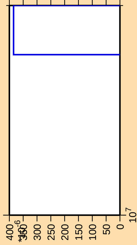
\Delta\sigma/\sigma vs. E for ^{164}\text{Lu} (mt 11)
