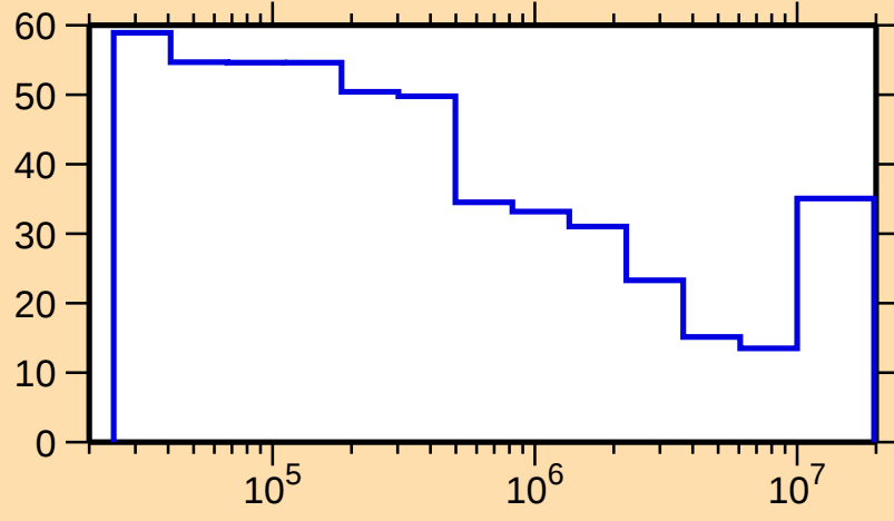
\Delta\sigma/\sigma vs. E for ^{164}\text{Lu}(n,\text{inel.})
