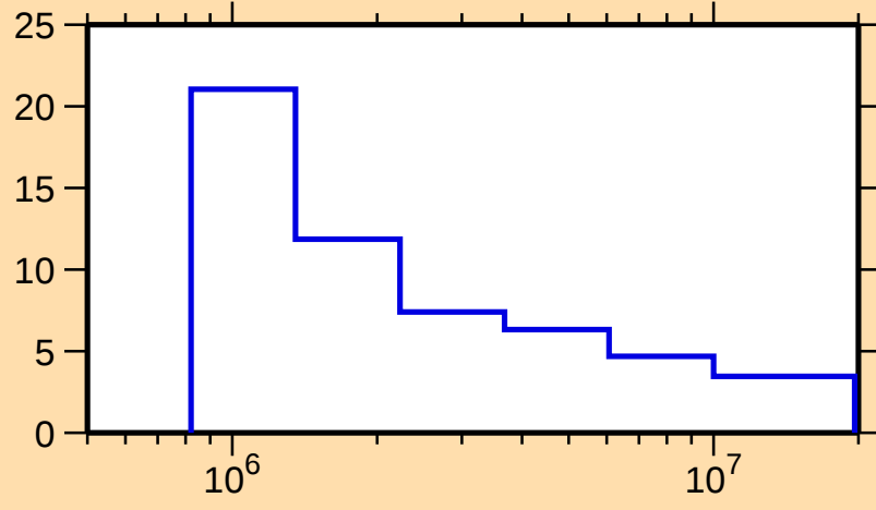
\Delta\sigma/\sigma vs. E for ^{164}\text{Lu}(n,\text{nonel.})
