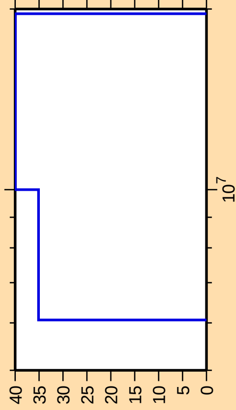
\Delta\sigma/\sigma vs. E for ^{164}\text{Lu}(n,n_1)
