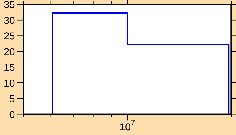
\Delta\sigma/\sigma vs. E for ^{164}\text{Lu}(n,2n)
