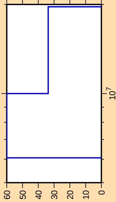
\Delta\sigma/\sigma vs. E for ^{164}\text{Lu}(n,p)
