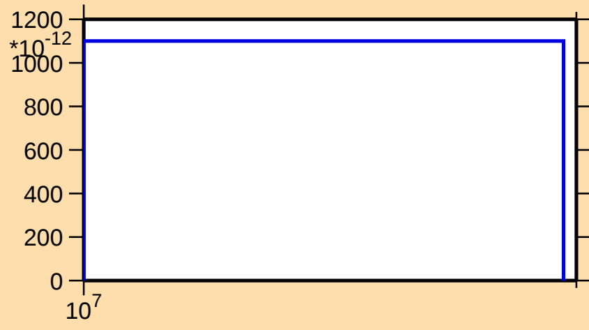
\sigma vs. E for ^{164}\text{Lu}(n,nt)
