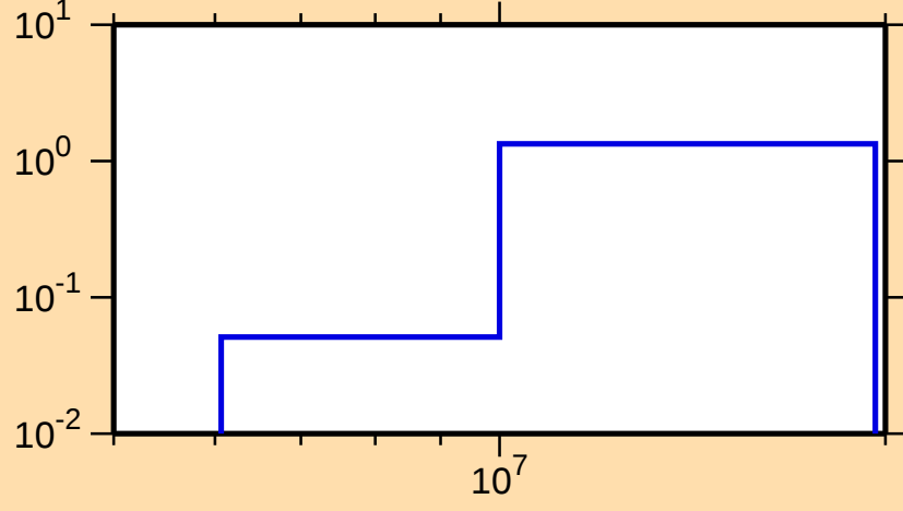
\sigma vs. E for ^{164}\text{Lu}(n,2n)
