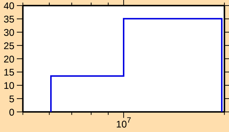
\Delta\sigma/\sigma vs. E for ^{164}\text{Lu}(n,\text{inel.})
