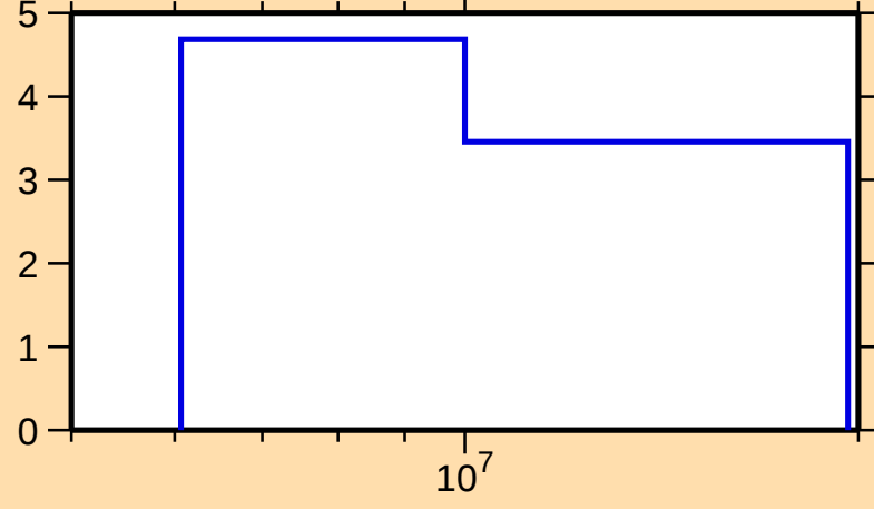
\Delta\sigma/\sigma vs. E for ^{164}\text{Lu}(n,\text{nonel.})
