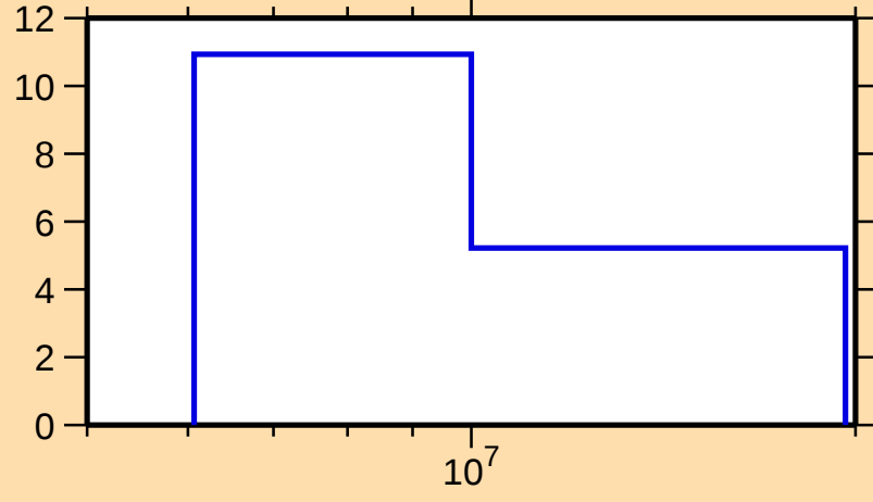
\Delta\sigma/\sigma vs. E for ^{164}\text{Lu}(n,\text{el.})
