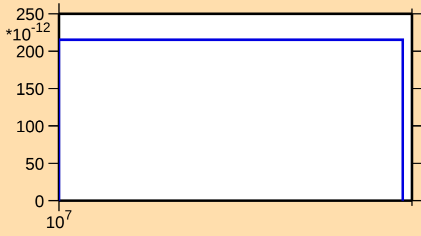
\sigma vs. E for ^{164}\text{Lu}(n,\text{pd})
