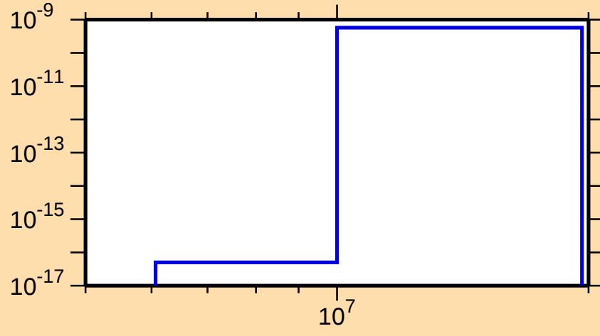
\sigma vs. E for ^{164}\text{Lu}(\text{mt117})
