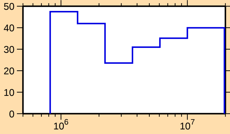
\Delta\sigma/\sigma vs. E for ^{164}\text{Lu}(n,n_1)
