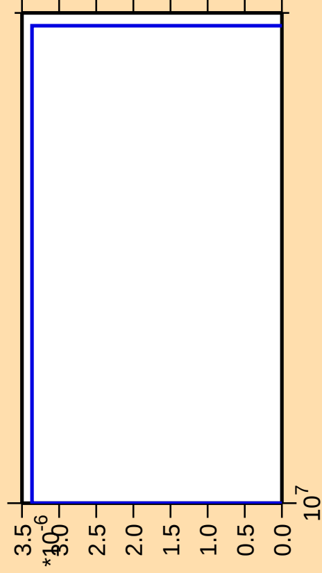
\Delta\sigma/\sigma vs. E for ^{164}\text{Lu}(\text{mt 11})
