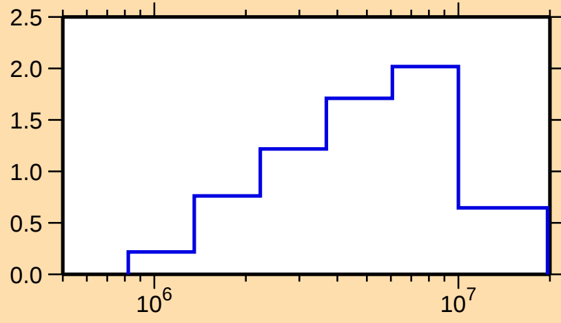
\sigma vs. E for ^{164}\text{Lu}(n,n\text{cont.})
