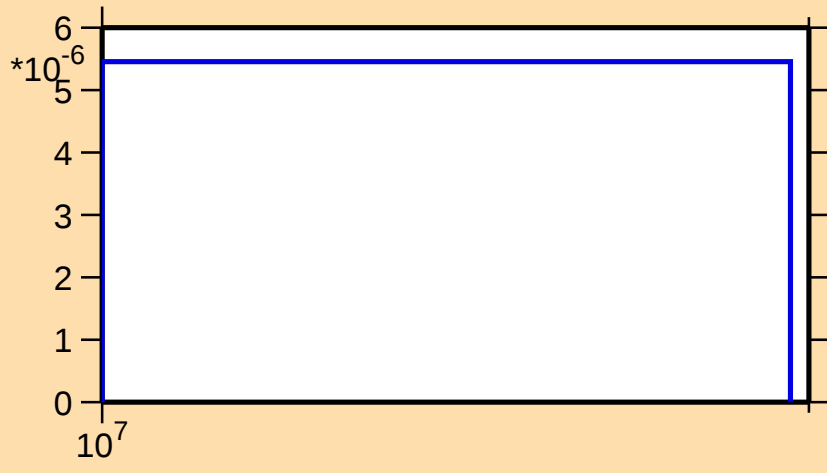
\sigma vs. E for ^{164}\text{Lu}(n,3n)
