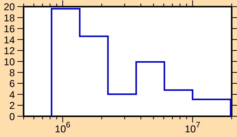
\Delta\sigma/\sigma vs. E for ^{164}\text{Lu}(n,\text{tot.})
