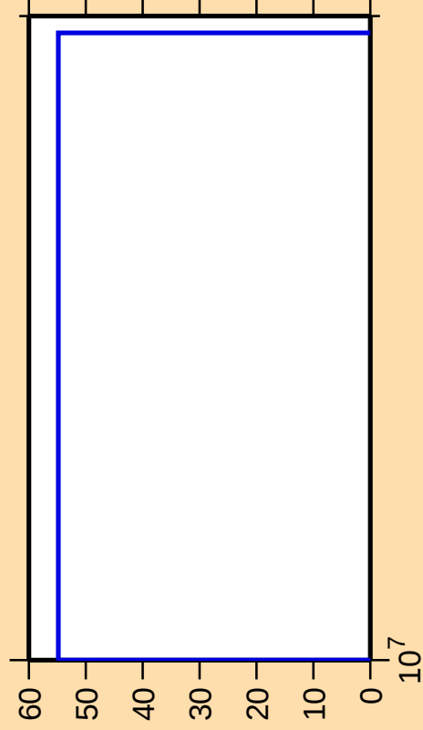
\Delta\sigma/\sigma vs. E for ^{164}\text{Lu} (mt 34)
