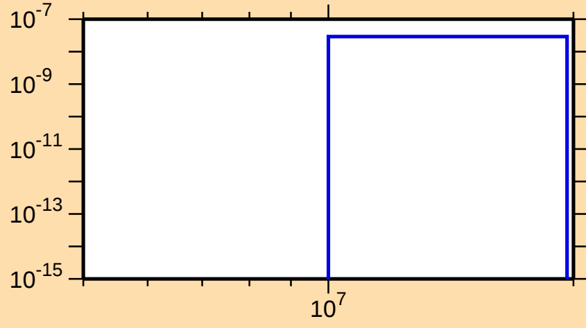
\sigma vs. E for ^{164}\text{Lu}(\text{mt 45})
