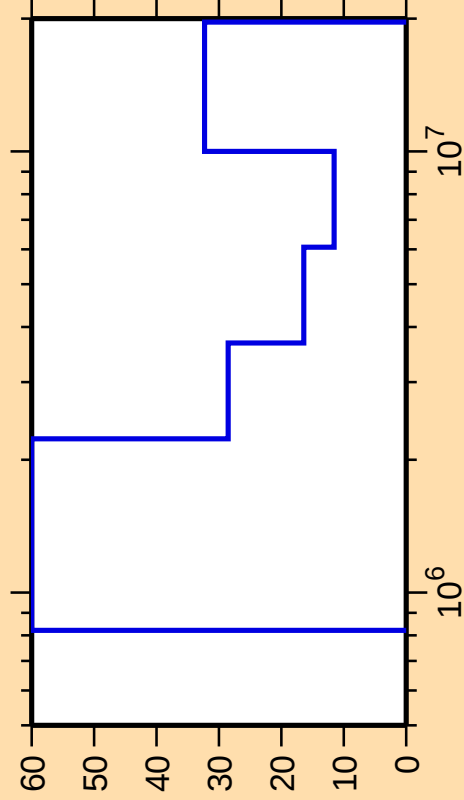
\Delta\sigma/\sigma vs. E for ^{164}\text{Lu}(n,n\text{cont.})
