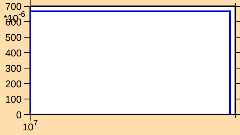
\sigma vs. E for ^{164}\text{Lu}(n,2np)
