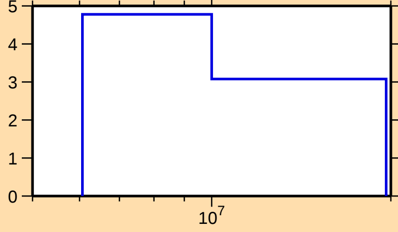
\Delta\sigma/\sigma vs. E for ^{164}\text{Lu}(n,\text{tot.})
