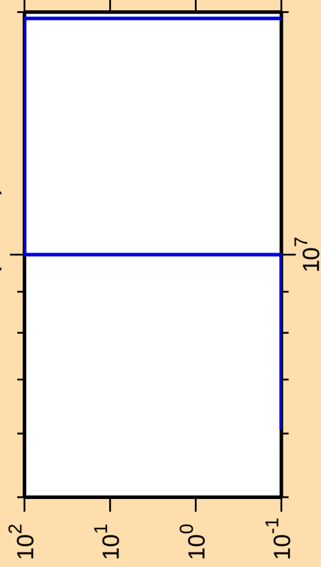
\Delta\sigma/\sigma vs. E for ^{164}\text{Lu}(\text{mt 45})
