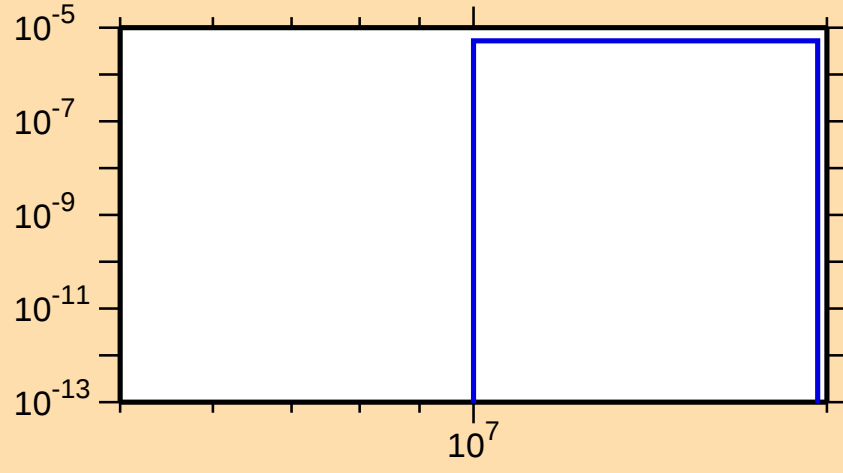
\sigma vs. E for ^{164}\text{Lu}(n,\text{nd})
