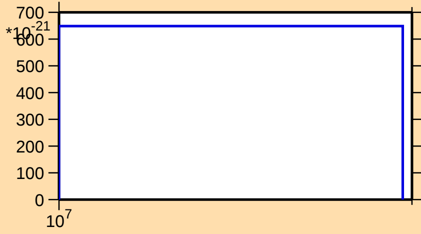
\sigma vs. E for ^{164}\text{Lu}(\text{mt 11})
