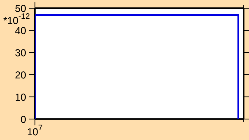
\sigma vs. E for ^{164}\text{Lu}(n,\text{pt})
