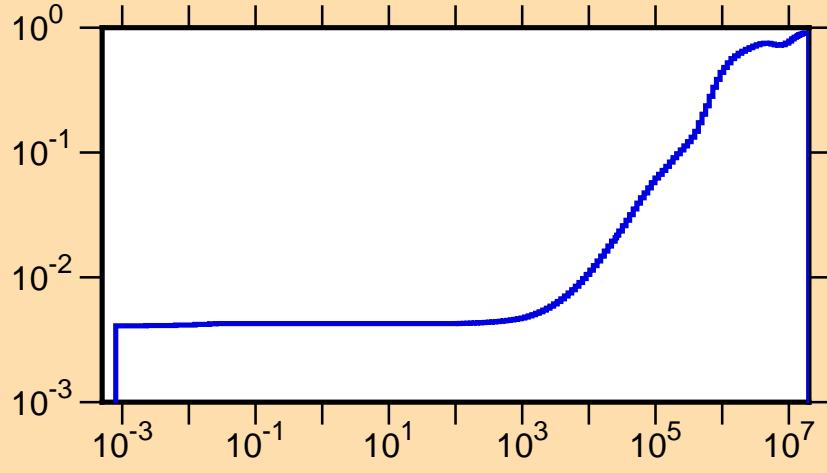
\mu vs. E for ^{165}\text{Lu}(\text{mt251})
