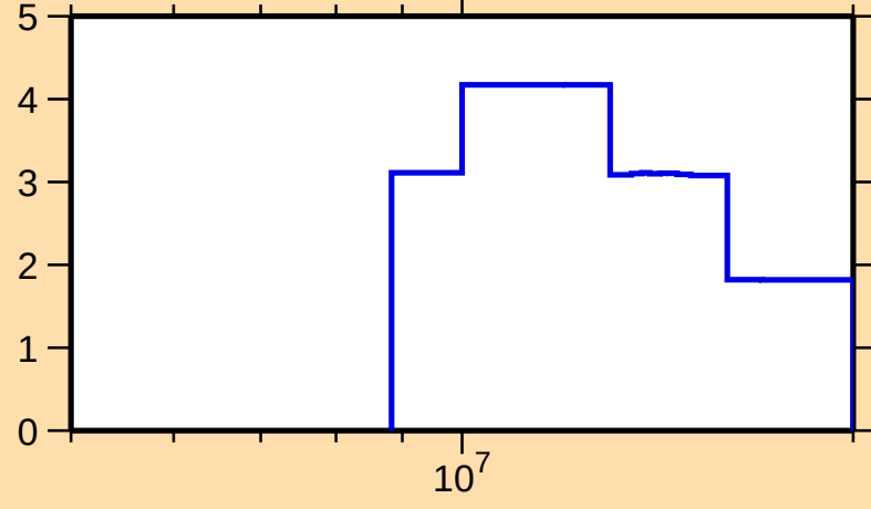
\Delta\sigma/\sigma vs. E for ^{165}\text{Lu}(n,\text{tot.})
