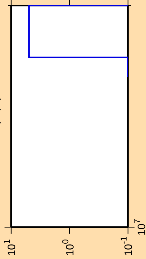
\Delta\sigma/\sigma vs. E for ^{165}\text{Lu}(n,\text{pt})
