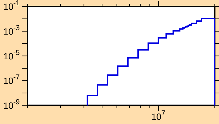
\sigma vs. E for ^{165}\text{Lu}(n,n\alpha)
