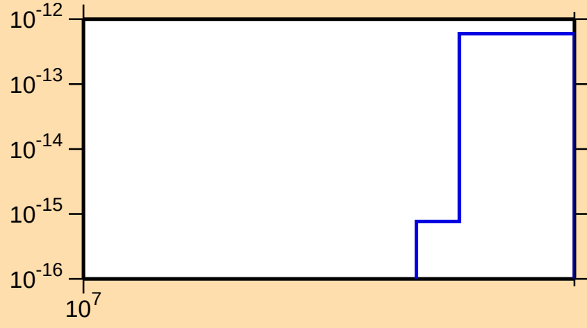
\sigma vs. E for ^{165}\text{Lu}(n,\text{pt})
