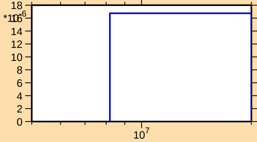
\sigma vs. E for ^{165}\text{Lu}(n,3n)
