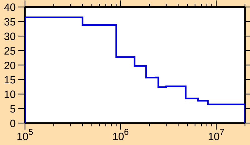
\Delta\sigma/\sigma vs. E for ^{165}\text{Lu}(n,\text{nonel.})
