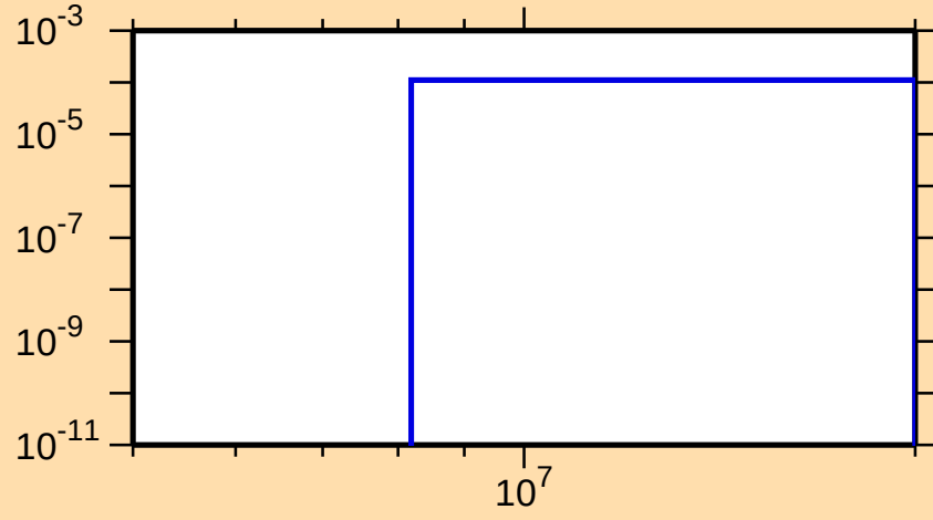
\sigma vs. E for ^{165}\text{Lu}(n,t)
