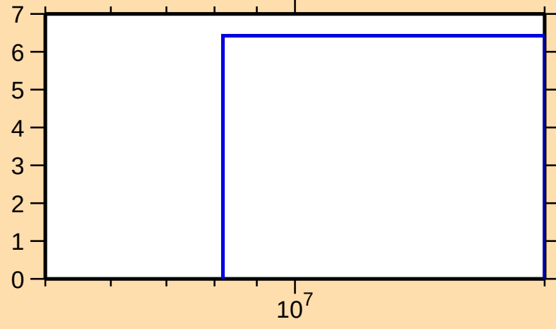
\Delta\sigma/\sigma vs. E for ^{165}\text{Lu}(n,\text{nonel.})
