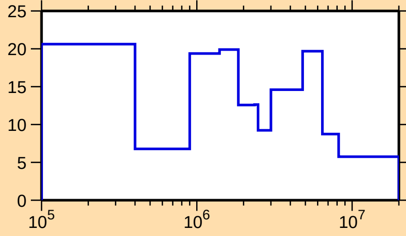
\Delta\sigma/\sigma vs. E for ^{165}\text{Lu}(\text{n,el.})
