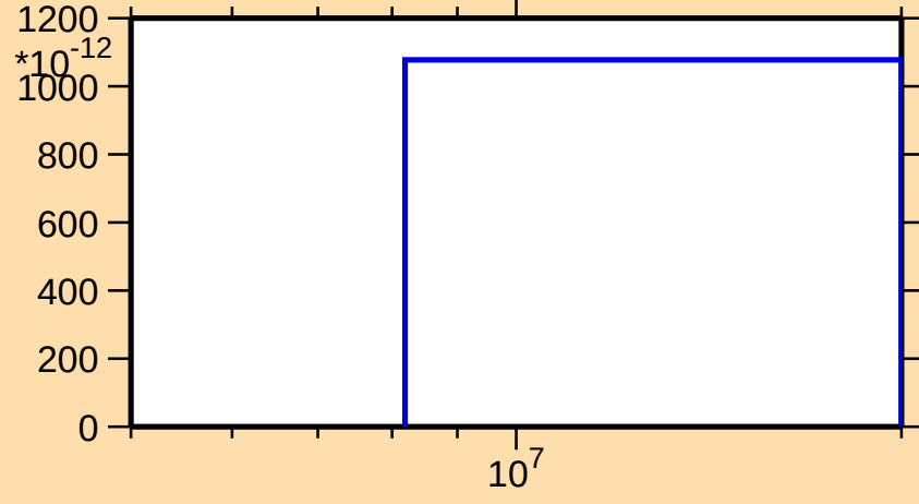
\sigma vs. E for ^{165}\text{Lu}(n,nt)
