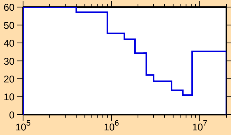
\Delta\sigma/\sigma vs. E for ^{165}\text{Lu}(n,n\text{cont.})
