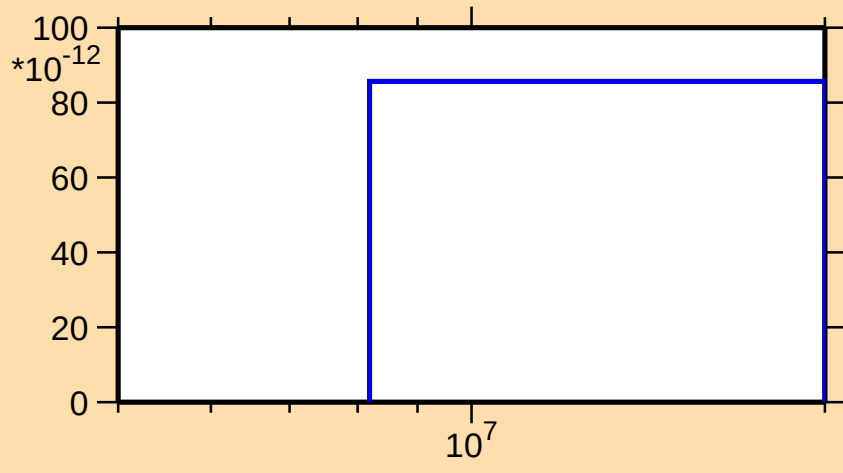
\sigma vs. E for ^{165}\text{Lu}(n,\text{pd})
