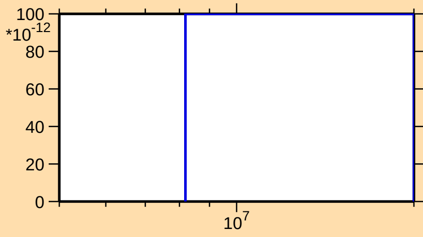
\sigma vs. E for ^{165}\text{Lu}(\text{mt117})
