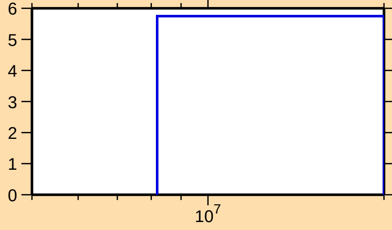
\Delta\sigma/\sigma vs. E for ^{165}\text{Lu}(n,\text{el.})
