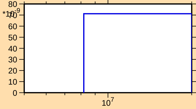
\sigma vs. E for ^{165}\text{Lu}(n,\text{nd})
