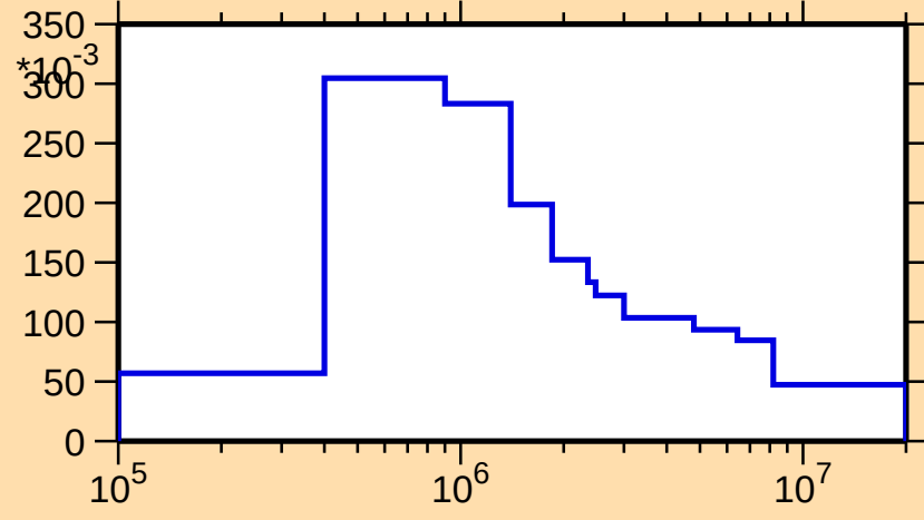
\sigma vs. E for ^{165}\text{Lu}(n,n_1)
