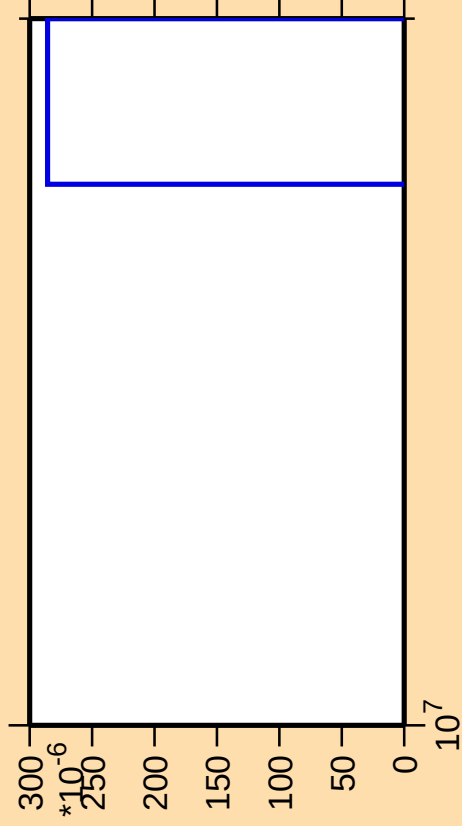
\Delta\sigma/\sigma vs. E for ^{166}\text{Lu} (mt 11)
