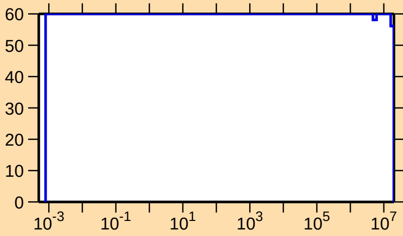
\Delta\sigma/\sigma vs. E for ^{166}\text{Lu}(n,p)
