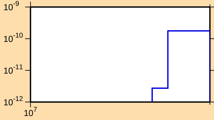
\sigma vs. E for ^{166}\text{Lu} (mt 34)
