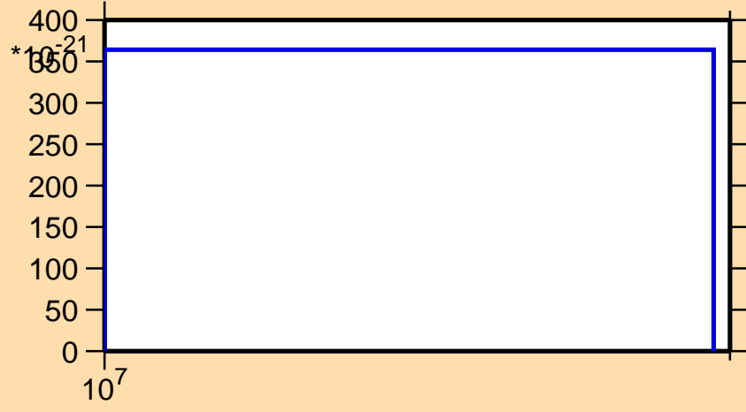
\sigma vs. E for ^{166}\text{Lu} (mt 11)
