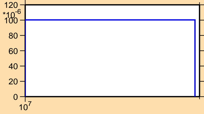
\sigma vs. E for ^{166}\text{Lu}(n,2np)
