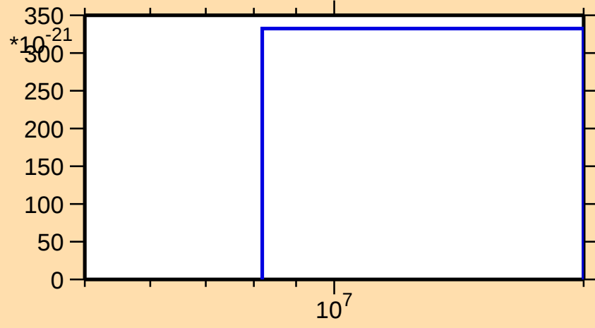
\sigma vs. E for ^{166}\text{Lu}(\text{mt 11})
