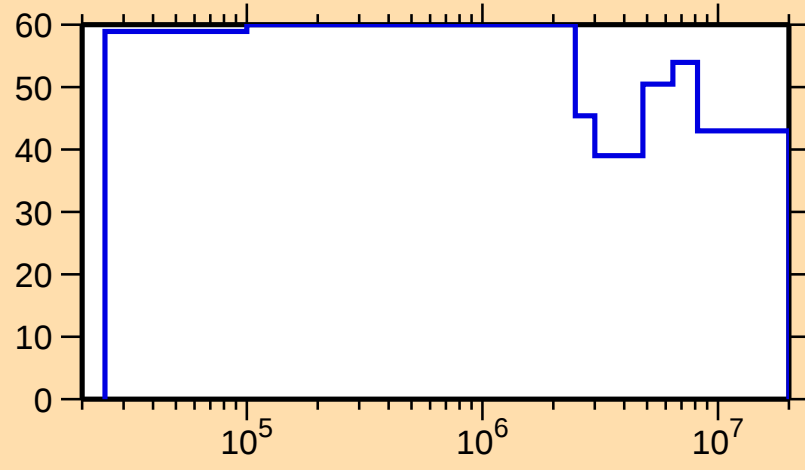
\Delta\sigma/\sigma vs. E for ^{166}\text{Lu}(n,n_1)
