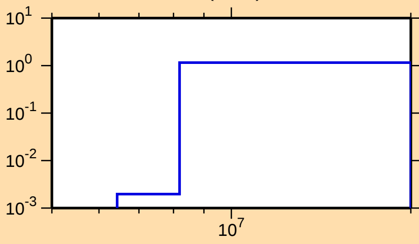
\sigma vs. E for ^{166}\text{Lu}(n,2n)
