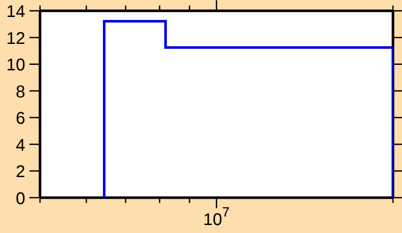
\Delta\sigma/\sigma vs. E for ^{166}\text{Lu}(n,\text{nonel.})
