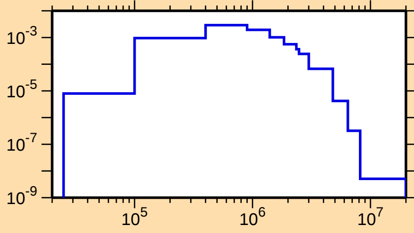
\sigma vs. E for ^{166}\text{Lu}(n,n_4)
