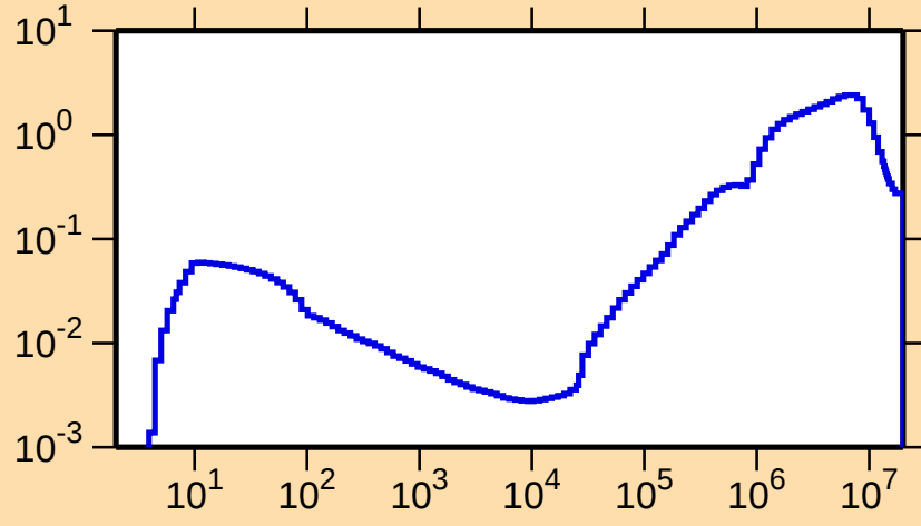
\sigma vs. E for ^{166}\text{Lu}(n,\text{inel.})
