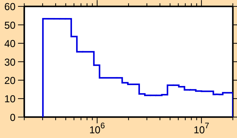
\Delta\sigma/\sigma vs. E for ^{166}\text{Lu}(n,n\text{onel.})
