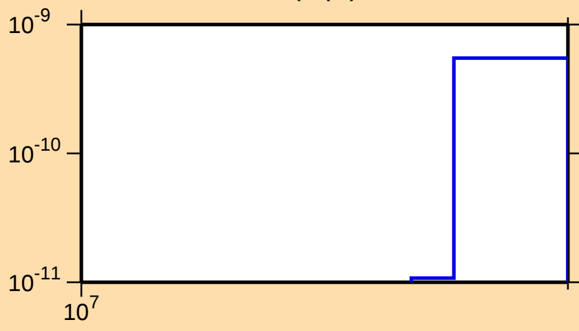
\sigma vs. E for ^{166}\text{Lu}(n,\text{pt})
