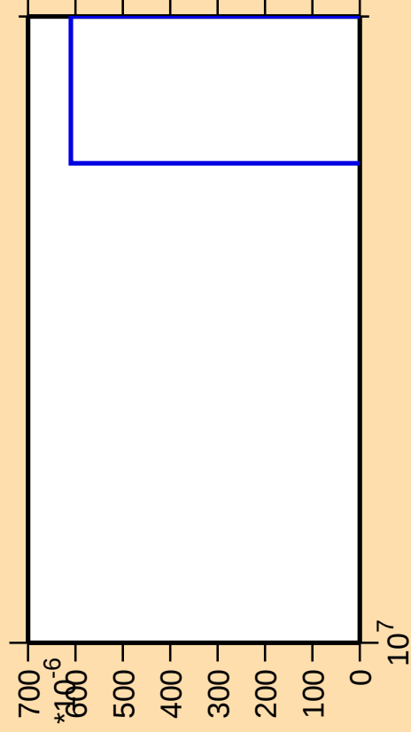
\Delta\sigma/\sigma vs. E for ^{166}\text{Lu} (mt 11)
