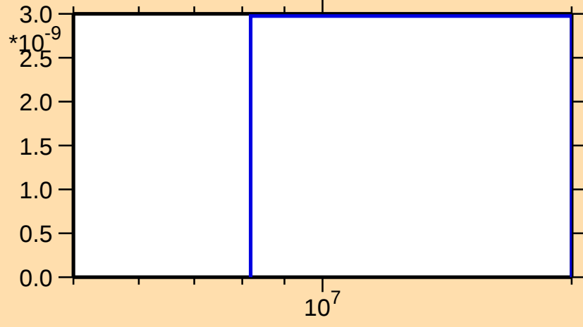
\sigma vs. E for ^{166}\text{Lu}(n,nt)
