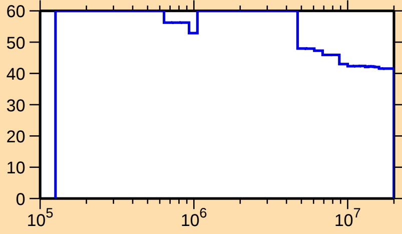
\Delta\sigma/\sigma vs. E for ^{167}\text{Lu}(n,n_1)
