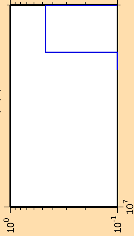
\Delta\sigma/\sigma vs. E for ^{167}\text{Lu}(n,\text{pt})
