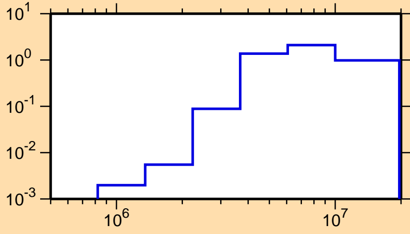
\sigma vs. E for ^{167}\text{Lu}(n,n\text{cont.})
