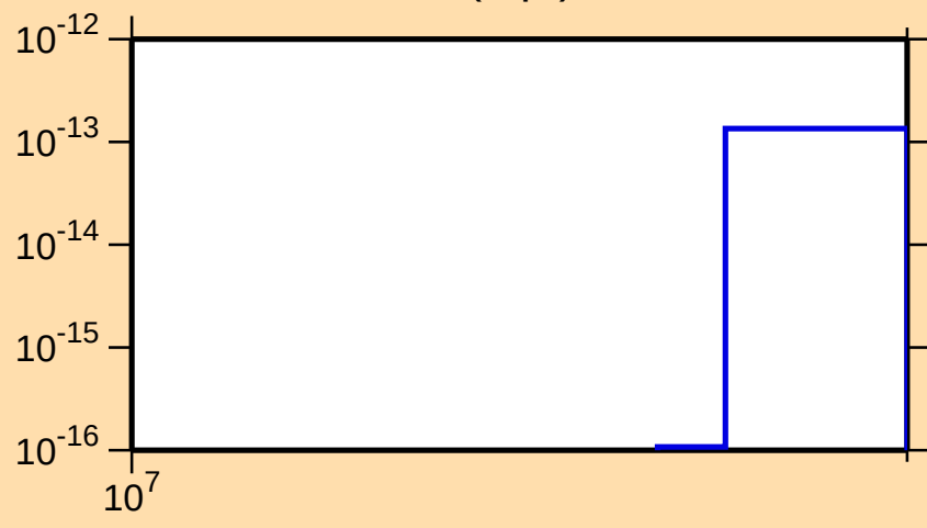
\sigma vs. E for ^{167}\text{Lu}(n,\text{pt})
