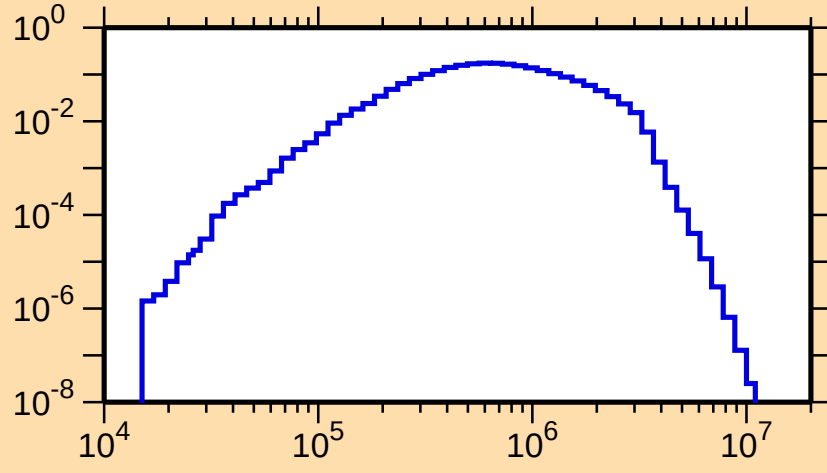
\sigma vs. E for ^{167}\text{Lu}(n,n_2)
