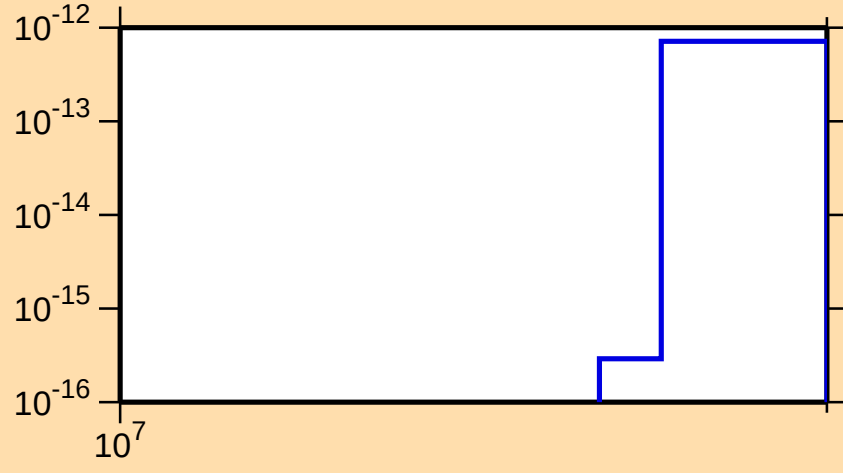
\sigma vs. E for ^{167}\text{Lu} (mt 34)
