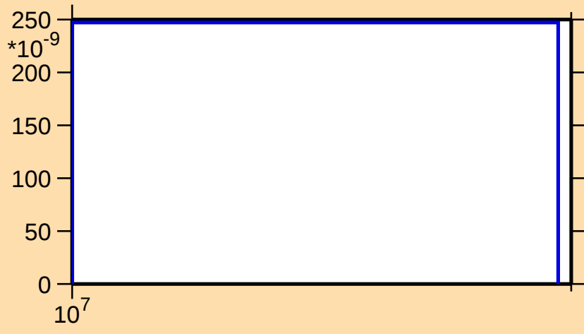
\sigma vs. E for ^{167}\text{Lu}(n,\text{nd})
