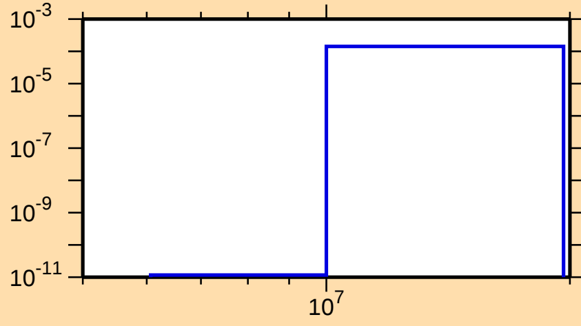
\sigma vs. E for ^{167}\text{Lu}(n,t)
