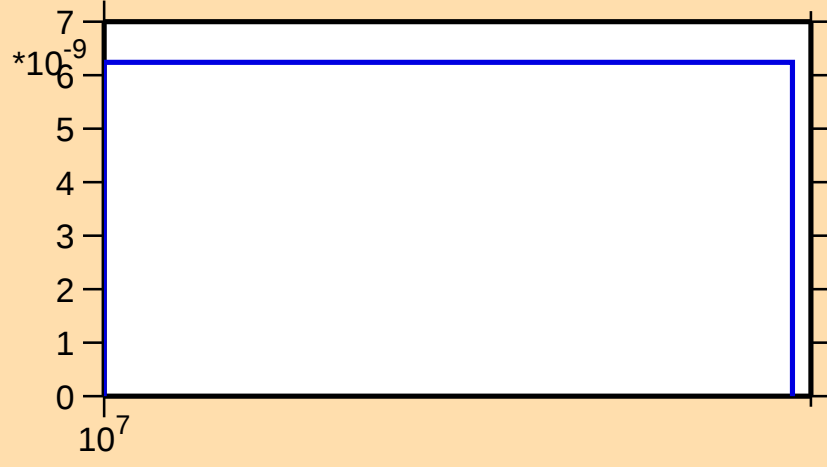
\sigma vs. E for ^{167}\text{Lu}(n,nt)
