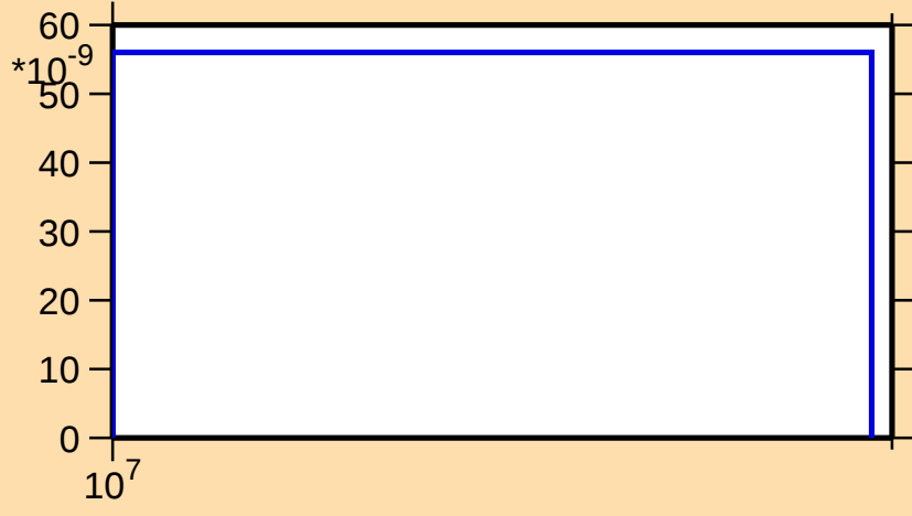
\sigma vs. E for ^{167}\text{Lu}(n,2n\alpha)
