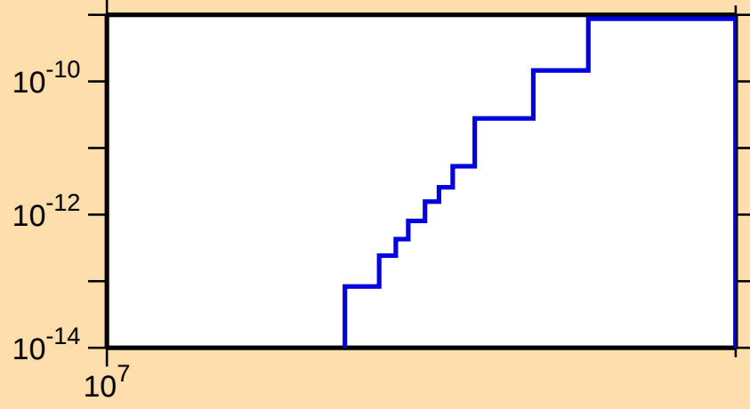
\sigma vs. E for ^{168}\text{Lu}(\text{mt } 45)
