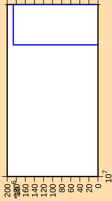
\Delta\sigma/\sigma vs. E for ^{168}\text{Lu} (mt 11)
