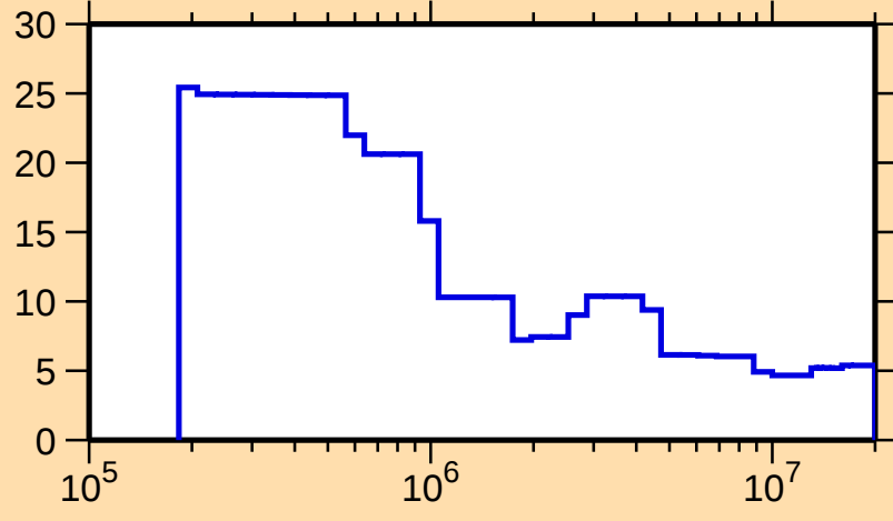
\Delta\sigma/\sigma vs. E for ^{168}\text{Lu}(n,\text{nonel.})
