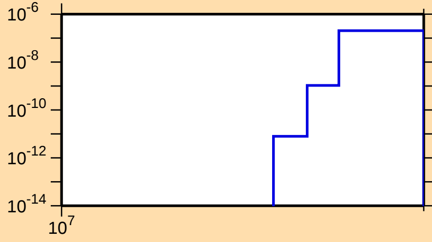
\sigma vs. E for ^{168}\text{Lu}(n,nt)
