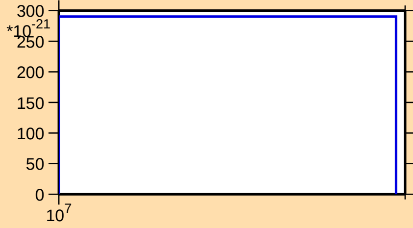
\sigma vs. E for ^{168}\text{Lu} (mt 11)
