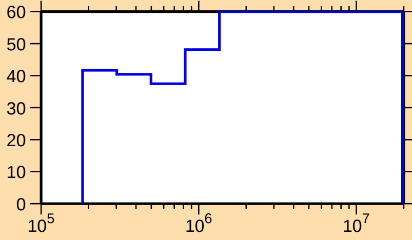
\Delta\sigma/\sigma vs. E for ^{168}\text{Lu}(n,n_1)
