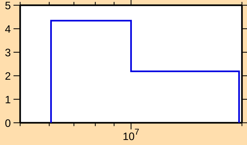
\Delta\sigma/\sigma vs. E for ^{168}\text{Lu}(n,\text{tot.})
