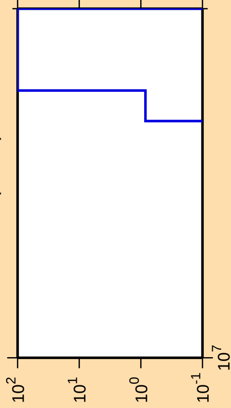
\Delta\sigma/\sigma vs. E for ^{168}\text{Lu} (mt 34)
