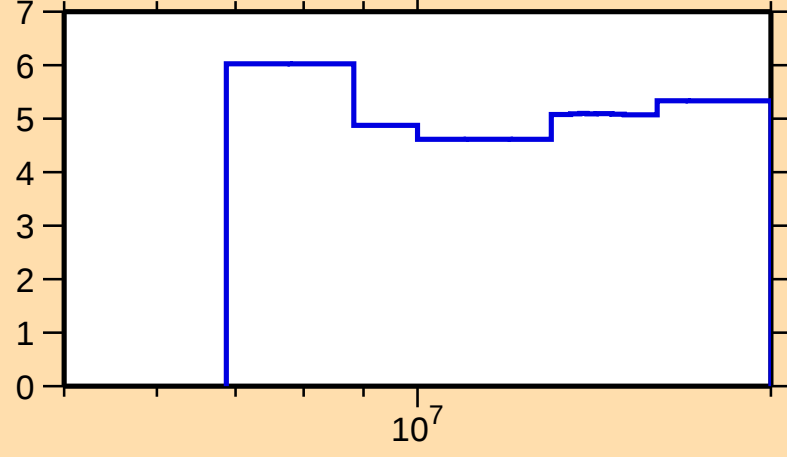
\Delta\sigma/\sigma vs. E for ^{168}\text{Lu}(n,\text{nonel.})
