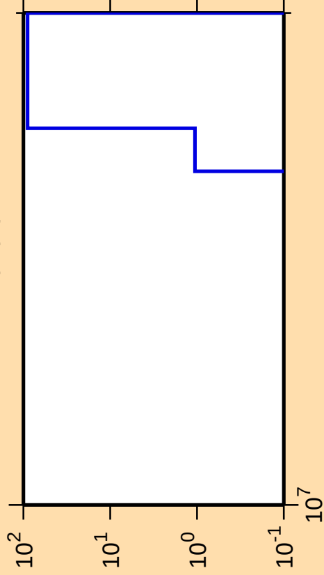
\Delta\sigma/\sigma vs. E for ^{168}\text{Lu}(n,\text{pt})
