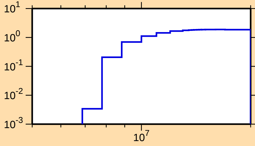
\sigma vs. E for ^{168}\text{Lu}(n,2n)
