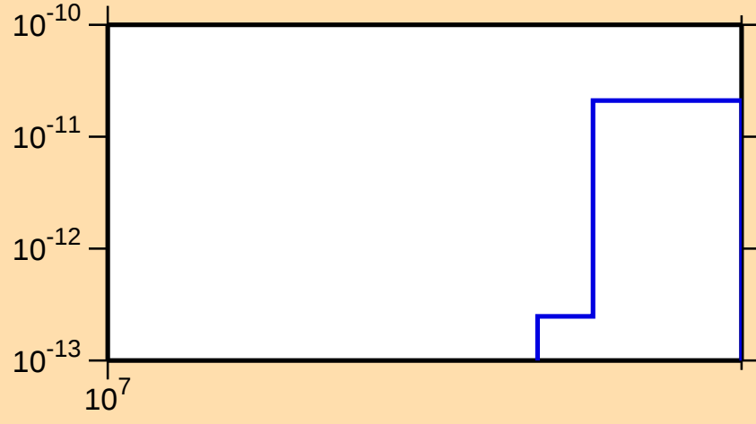
\sigma vs. E for ^{168}\text{Lu}(n,\text{pt})
