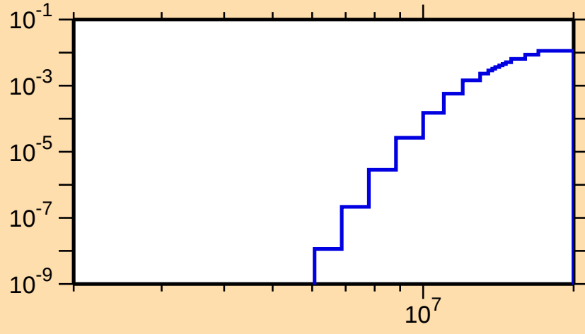
\sigma vs. E for ^{168}\text{Lu}(n,d)
