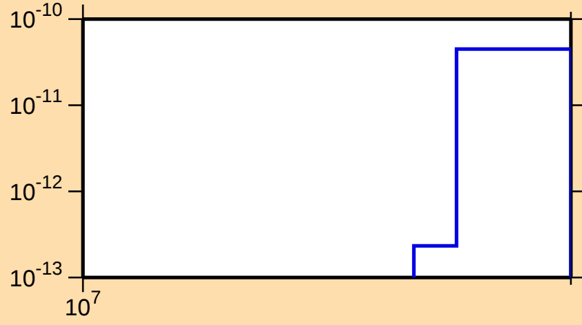
\sigma vs. E for ^{168}\text{Lu} (mt 34)
