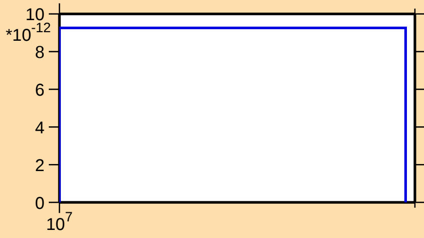
\sigma vs. E for ^{168}\text{Lu}(\text{mt117})
