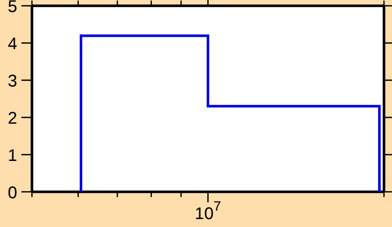
\Delta\sigma/\sigma vs. E for ^{168}\text{Lu}(n,\text{tot.})
