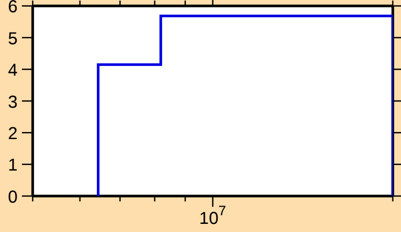
\Delta\sigma/\sigma vs. E for ^{168}\text{Lu}(n,\text{el.})
