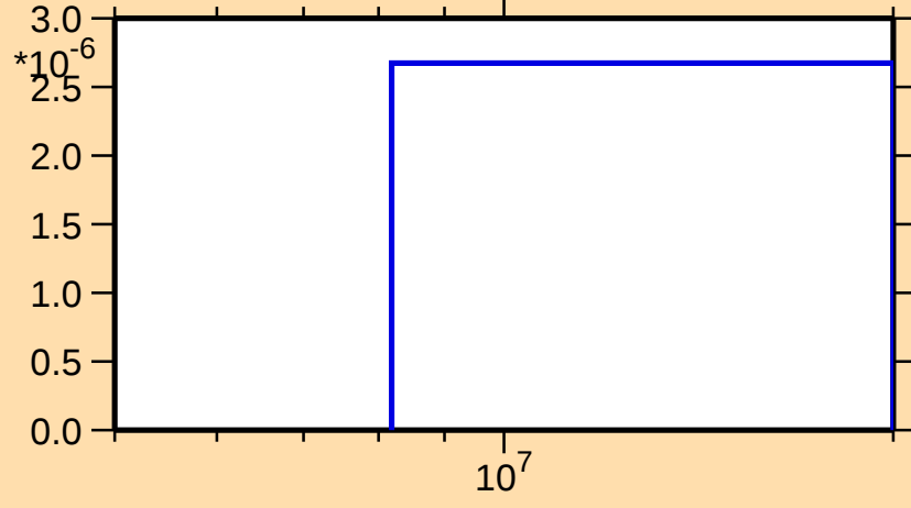
\sigma vs. E for ^{168}\text{Lu}(n,\text{nd})
