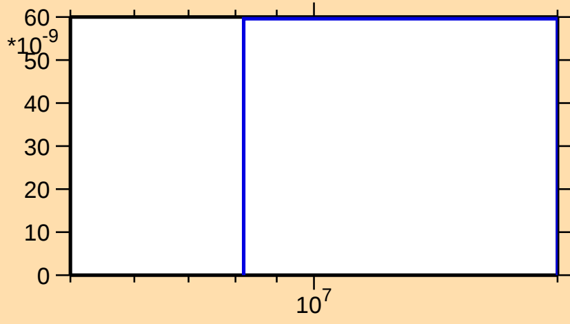
\sigma vs. E for ^{168}\text{Lu}(n,\text{He}3)
