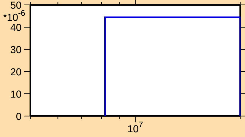
\sigma vs. E for ^{168}\text{Lu}(n,2np)
