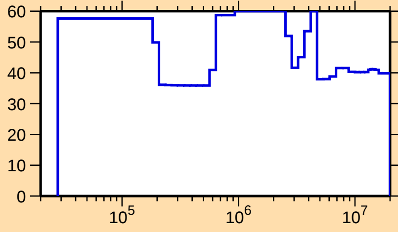
\Delta\sigma/\sigma vs. E for ^{169}\text{Lu}(n,n_1)
