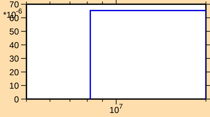
\sigma vs. E for ^{169}\text{Lu}(n,t)
