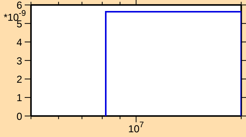
\sigma vs. E for ^{169}\text{Lu}(n,2n\alpha)
