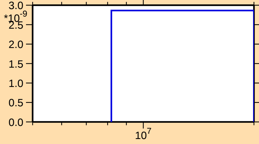
\sigma vs. E for ^{169}\text{Lu}(n,nt)
