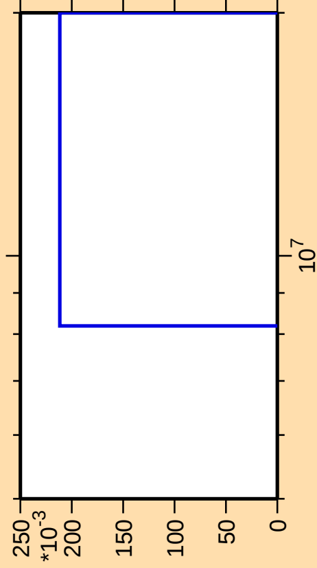
\Delta\sigma/\sigma vs. E for ^{169}\text{Lu}(n,\text{pd})
