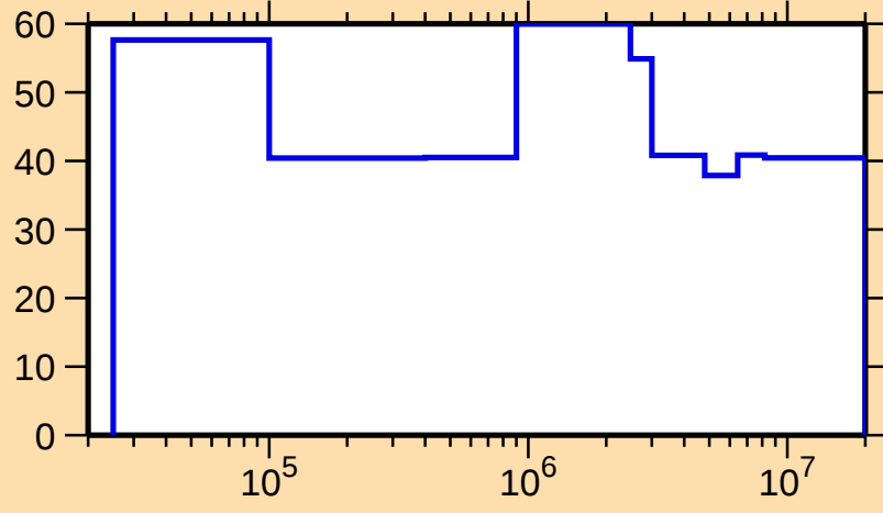
\Delta\sigma/\sigma vs. E for ^{169}\text{Lu}(n,n_1)
