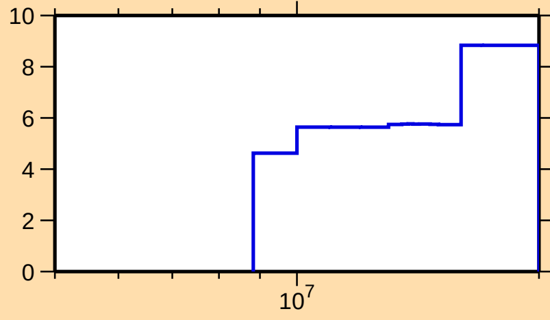
\Delta\sigma/\sigma vs. E for ^{169}\text{Lu}(n,\text{tot.})
