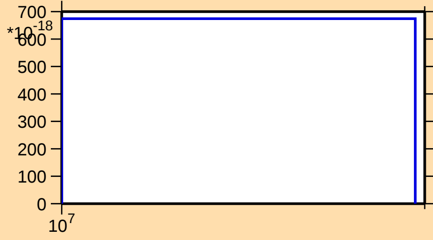
\sigma vs. E for ^{169}\text{Lu} (mt 34)
