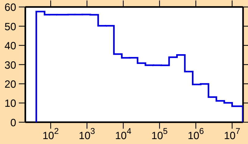
\Delta\sigma/\sigma vs. E for ^{169}\text{Lu}(n,\text{nonel.})
