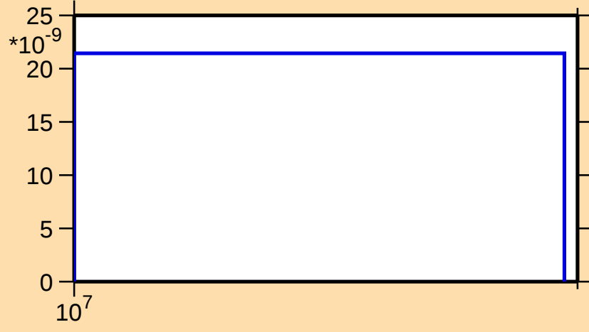
\sigma vs. E for ^{169}\text{Lu}(n,2n\alpha)
