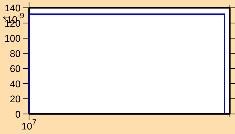
\sigma vs. E for ^{169}\text{Lu}(n,\text{nd})
