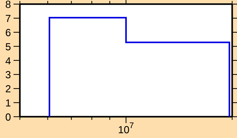
\Delta\sigma/\sigma vs. E for ^{169}\text{Lu}(n,\text{tot.})
