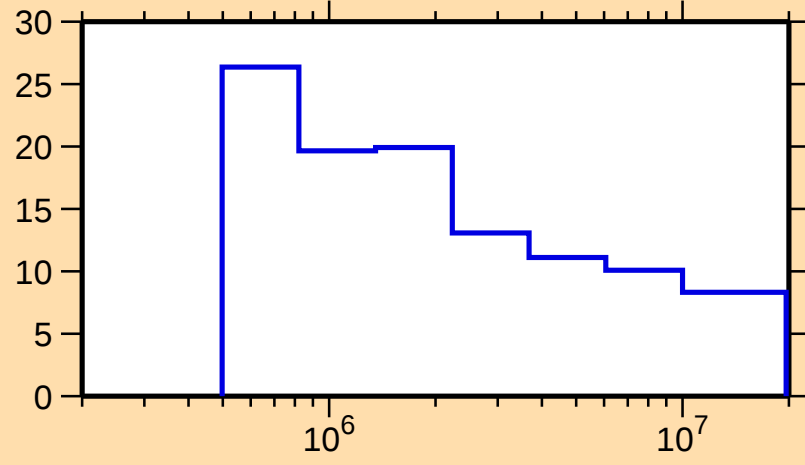
\Delta\sigma/\sigma vs. E for ^{169}\text{Lu}(n,n\text{onel.})
