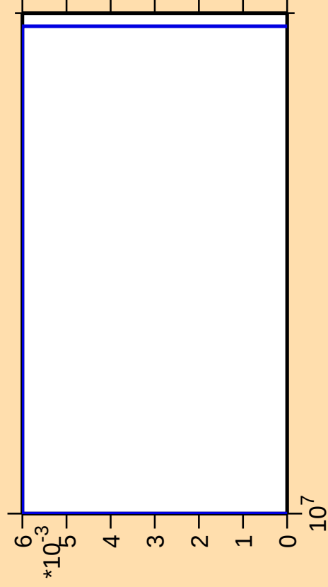
\Delta\sigma/\sigma vs. E for ^{169}\text{Lu} (mt 34)
