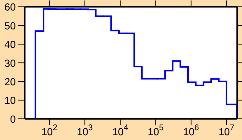
\Delta\sigma/\sigma vs. E for ^{169}\text{Lu}(n,\text{el.})
