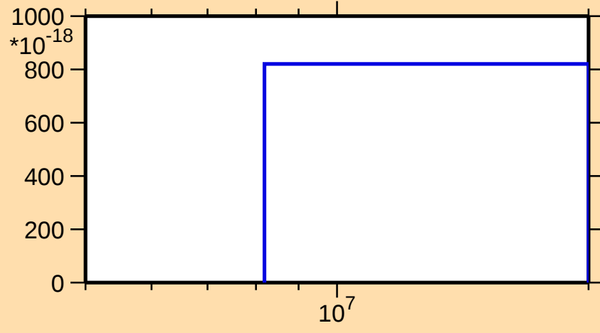
\sigma vs. E for ^{169}\text{Lu}(\text{mt } 34)
