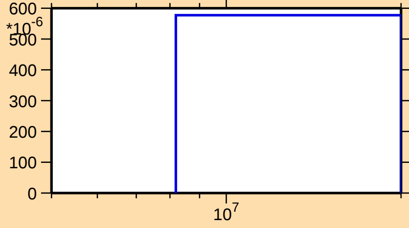
\sigma vs. E for ^{169}\text{Lu}(n,3n)
