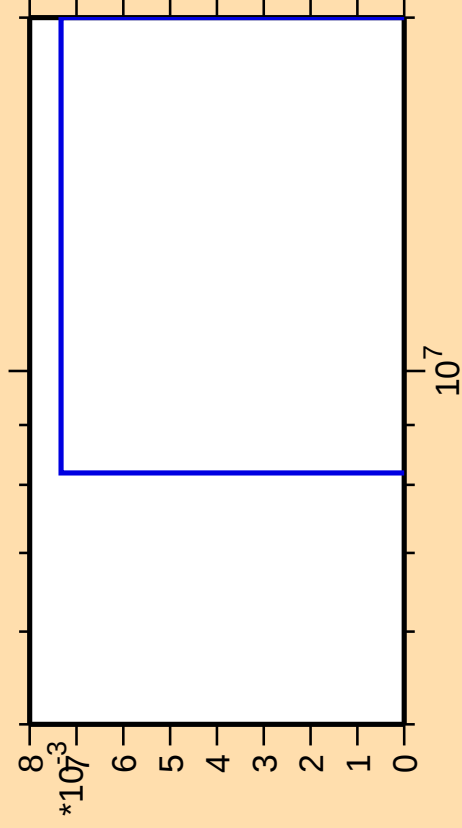
\Delta\sigma/\sigma vs. E for ^{169}\text{Lu}(\text{mt } 34)
