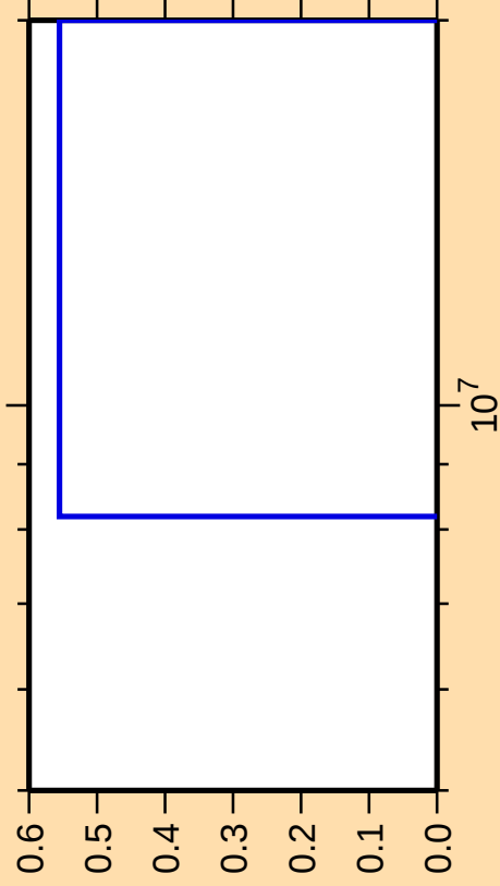
\Delta\sigma/\sigma vs. E for ^{169}\text{Lu}(n,\text{pd})
