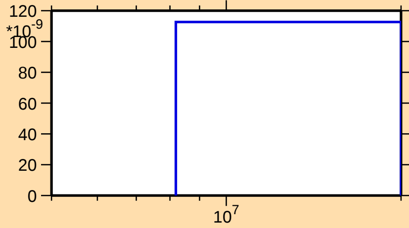
\sigma vs. E for ^{169}\text{Lu}(n,\text{nd})
