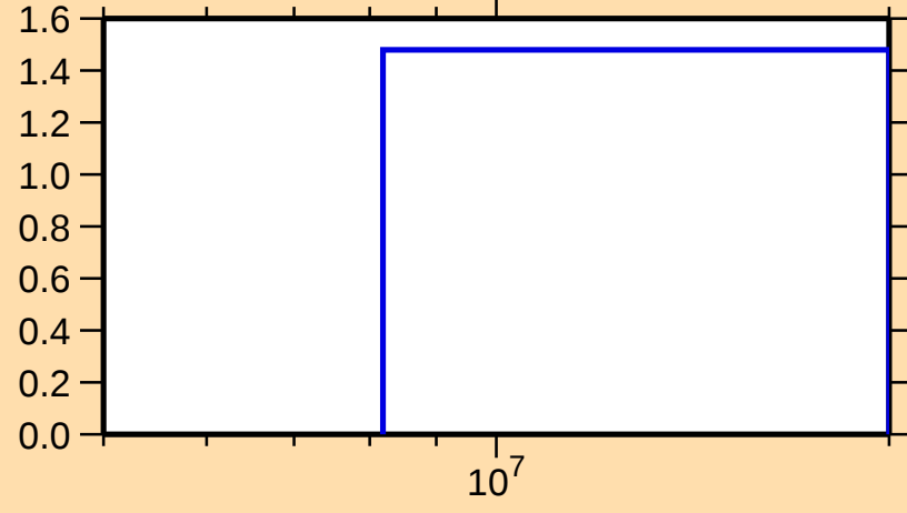
\sigma vs. E for ^{169}\text{Lu}(n,2n)
