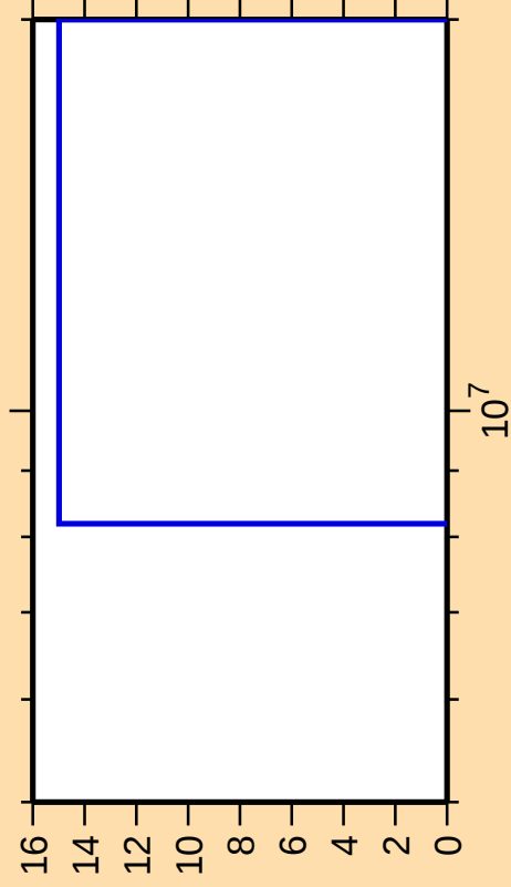
\Delta\sigma/\sigma vs. E for ^{169}\text{Lu}(n,2n)
