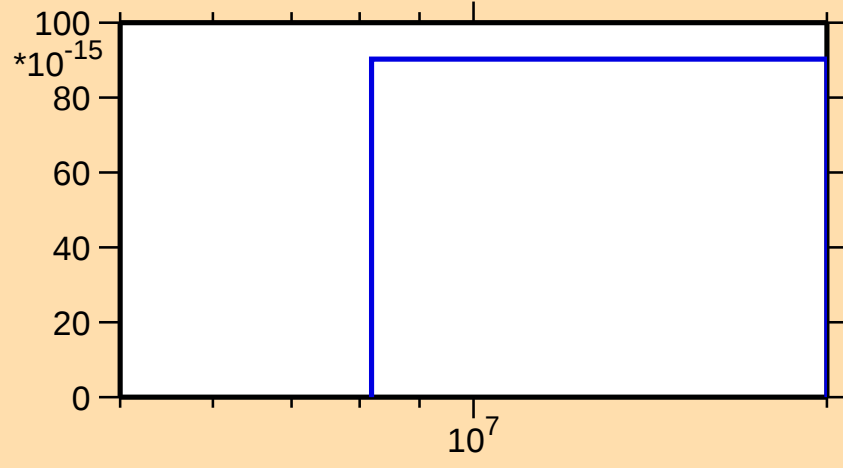
\sigma vs. E for ^{169}\text{Lu}(n,\text{pd})
