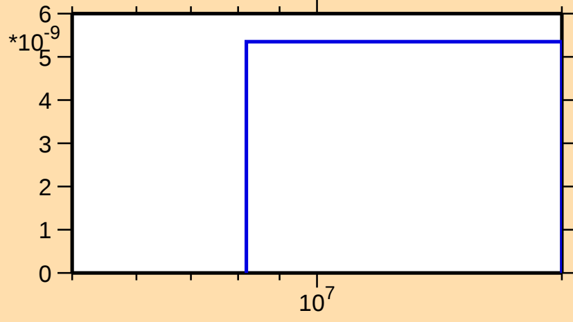
\sigma vs. E for ^{169}\text{Lu}(n,nt)
