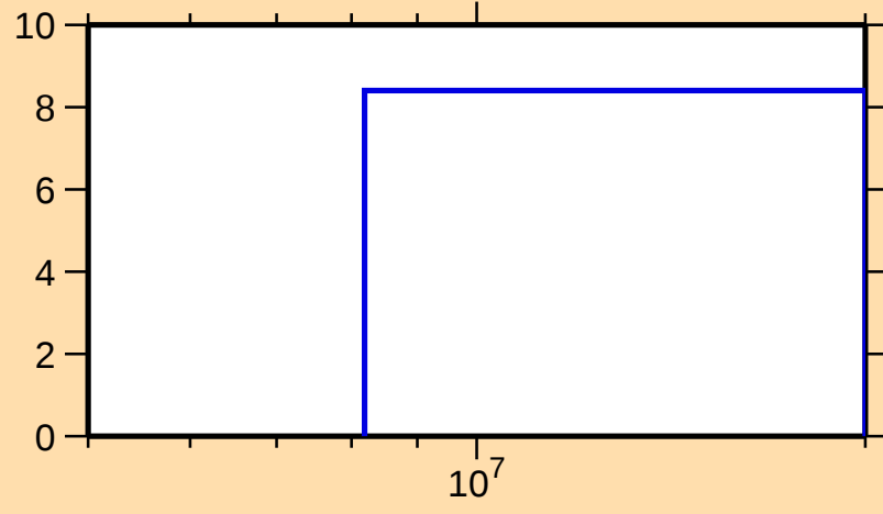
\Delta\sigma/\sigma vs. E for ^{169}\text{Lu}(n,\text{nonel.})
