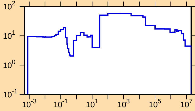
\Delta\sigma/\sigma vs. E for ^{169}\text{Lu}(n,\text{tot.})
