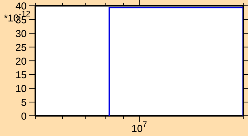
\sigma vs. E for ^{169}\text{Lu} (mt 45)
