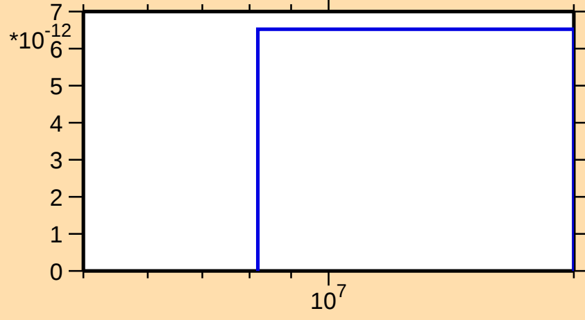
\sigma vs. E for ^{169}\text{Lu}(\text{mt117})
