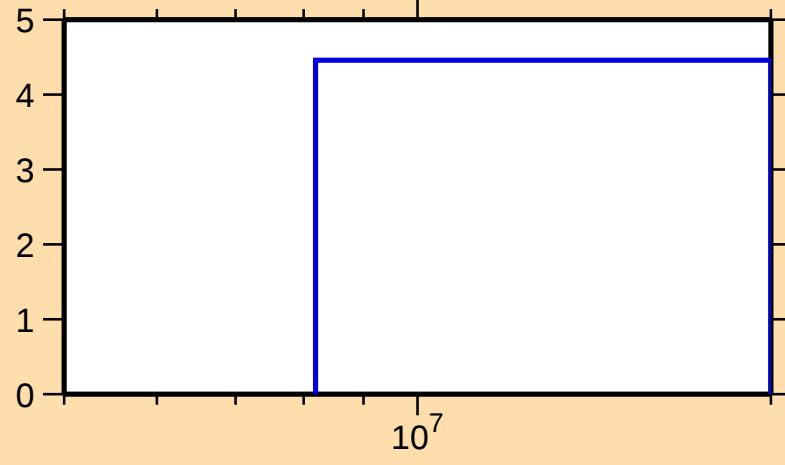
\Delta\sigma/\sigma vs. E for ^{169}\text{Lu}(n,\text{tot.})
