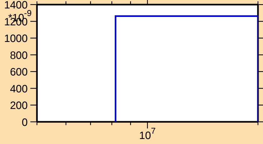
\sigma vs. E for ^{169}\text{Lu}(n,2np)
