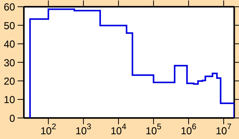
\Delta\sigma/\sigma vs. E for ^{169}\text{Lu}(n,\text{el.})
