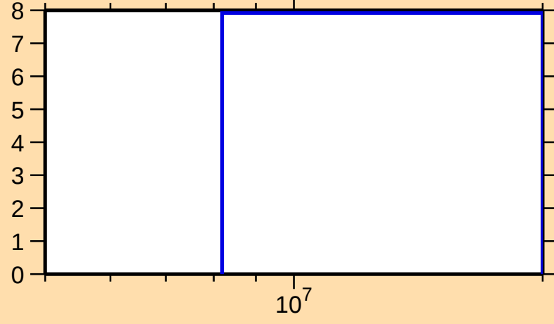
\Delta\sigma/\sigma vs. E for ^{169}\text{Lu}(n,\text{el.})
