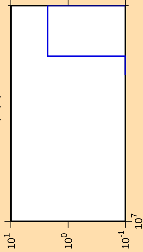
\Delta\sigma/\sigma vs. E for ^{170}\text{Lu}(n,\text{pt})
