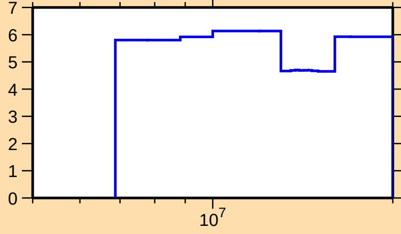
\Delta\sigma/\sigma vs. E for ^{170}\text{Lu}(n,\text{tot.})
