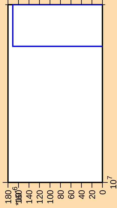
\Delta\sigma/\sigma vs. E for ^{170}\text{Lu} (mt 11)
