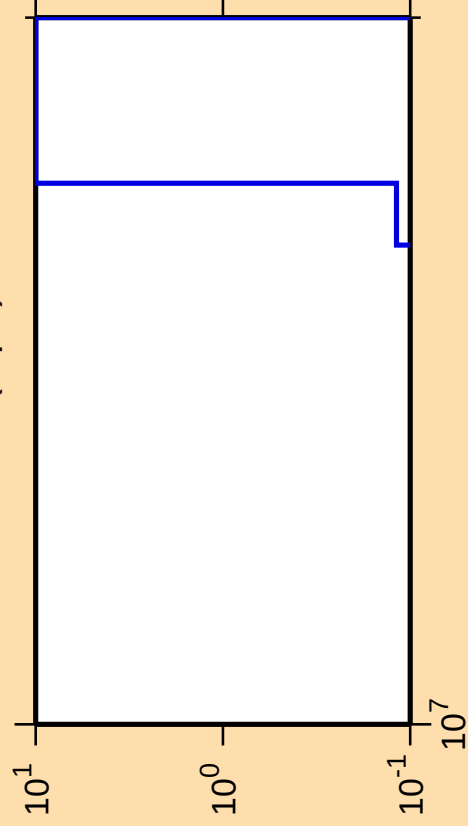
\Delta\sigma/\sigma vs. E for ^{170}\text{Lu}(n,\text{pd})
