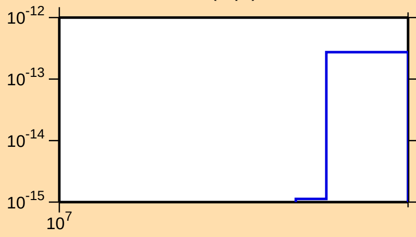
\sigma vs. E for ^{170}\text{Lu}(n,\text{pt})
