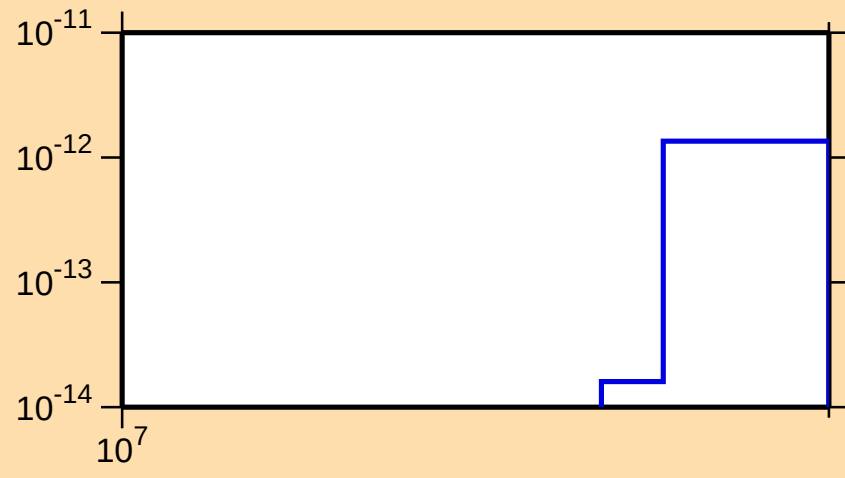
\sigma vs. E for ^{170}\text{Lu}(n,\text{pd})
