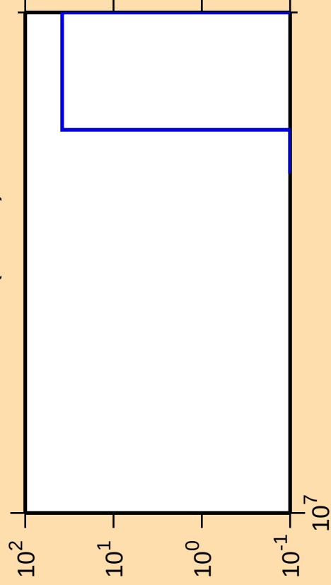
\Delta\sigma/\sigma vs. E for ^{170}\text{Lu} (mt 34)
