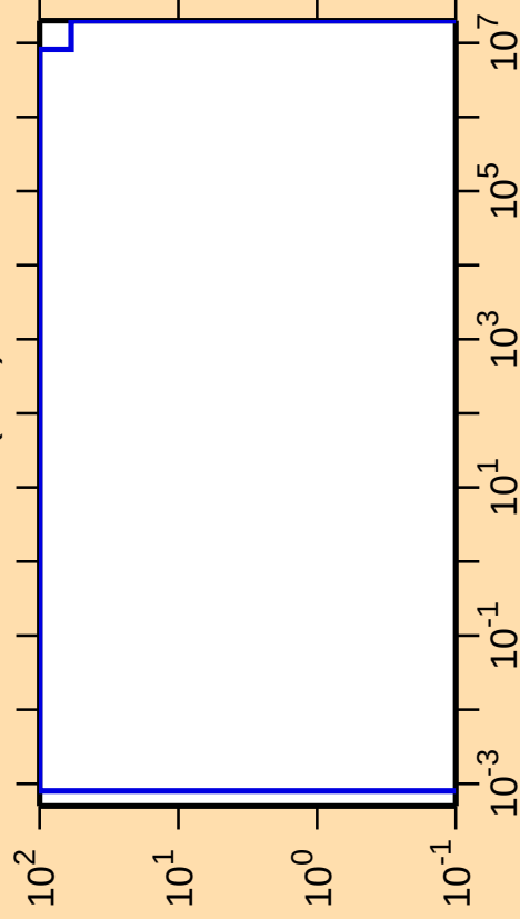
\Delta\sigma/\sigma vs. E for ^{171}\text{Lu}(n,\alpha)
