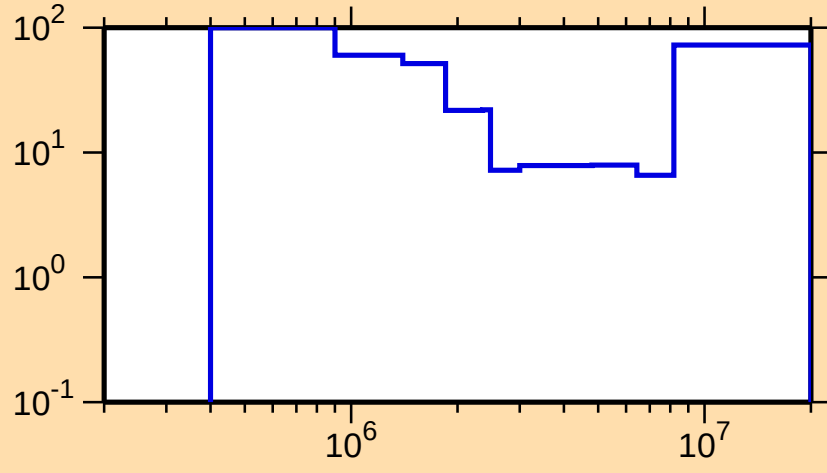
\Delta\sigma/\sigma vs. E for ^{171}\text{Lu}(n,n\text{cont.})
