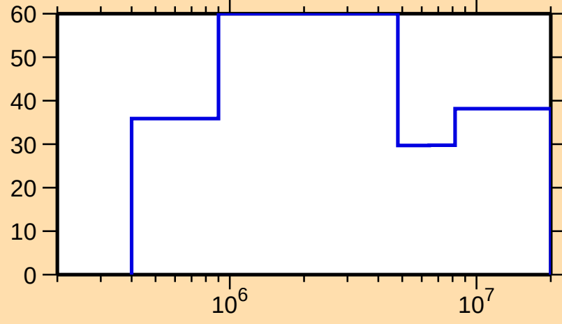
\Delta\sigma/\sigma vs. E for ^{171}\text{Lu}(n,n_1)
