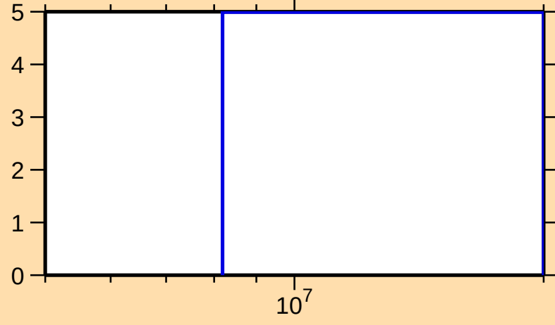
\Delta\sigma/\sigma vs. E for ^{171}\text{Lu}(n,\text{nonel.})
