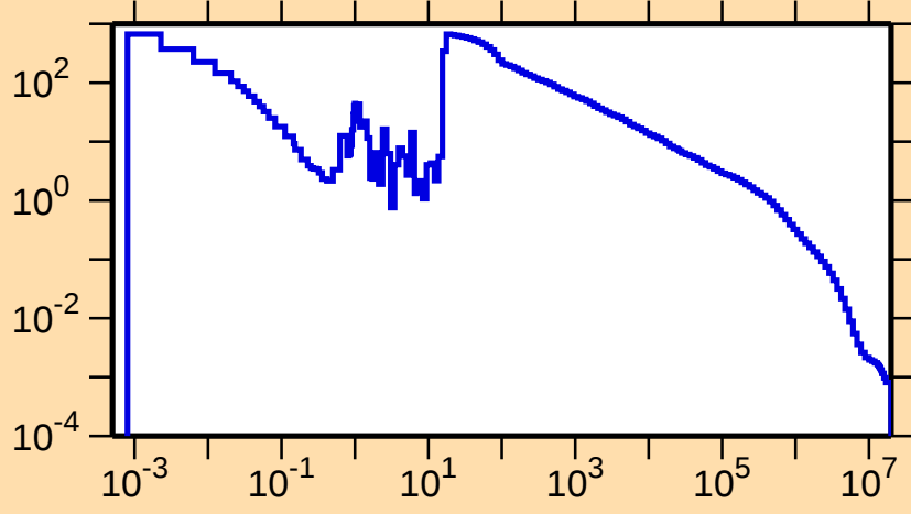
\sigma vs. E for ^{172}\text{Lu}(n,\gamma)
