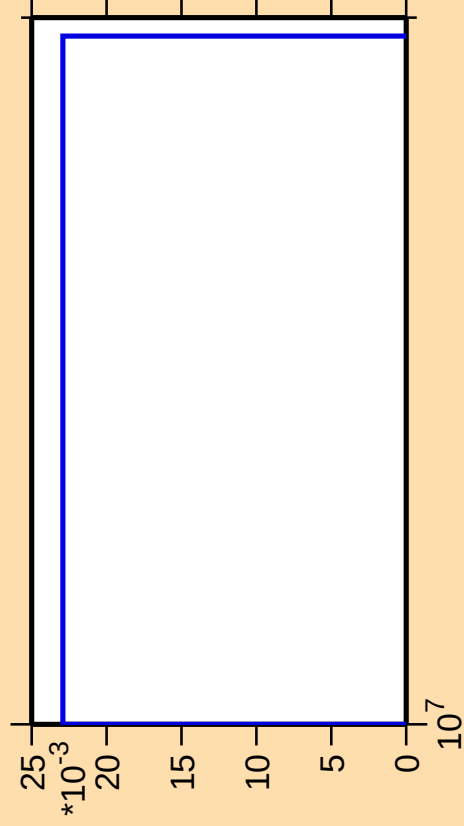
\Delta\sigma/\sigma vs. E for ^{172}\text{Lu} (mt 34)
