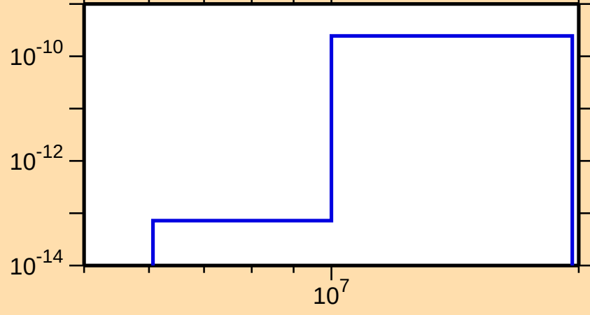
\sigma vs. E for ^{172}\text{Lu}(n,p\alpha)
