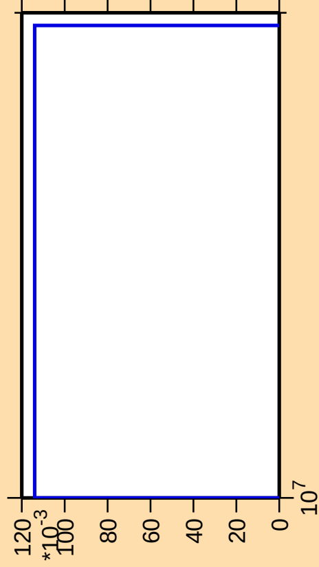
\Delta\sigma/\sigma vs. E for ^{172}\text{Lu} (mt 45)
