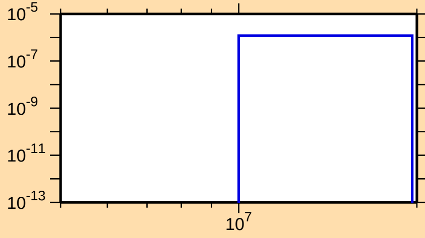
\sigma vs. E for ^{172}\text{Lu}(n,\text{nd})
