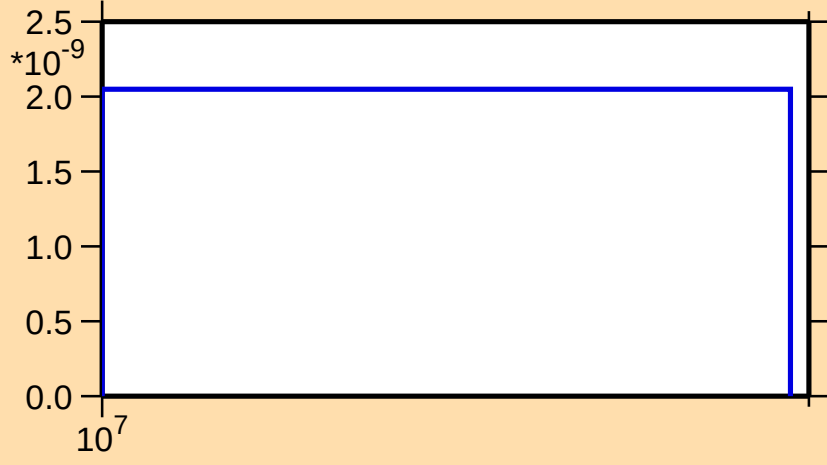
\sigma vs. E for ^{172}\text{Lu}(n,\text{He}3)
