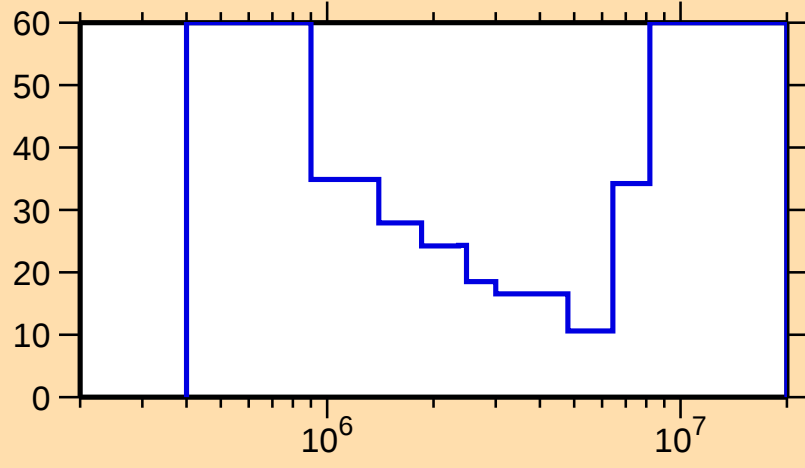
\Delta\sigma/\sigma vs. E for ^{172}\text{Lu}(n,\text{ncont.})
