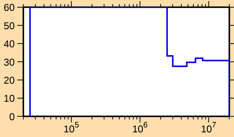
\Delta\sigma/\sigma vs. E for ^{172}\text{Lu}(n,n_1)
