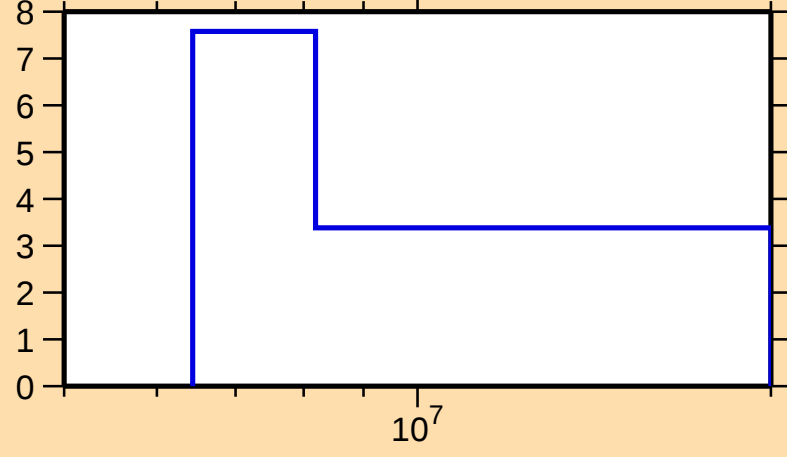
\Delta\sigma/\sigma vs. E for ^{172}\text{Lu}(n,\text{tot.})
