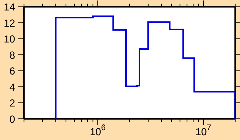
\Delta\sigma/\sigma vs. E for ^{172}\text{Lu}(n,\text{tot.})
