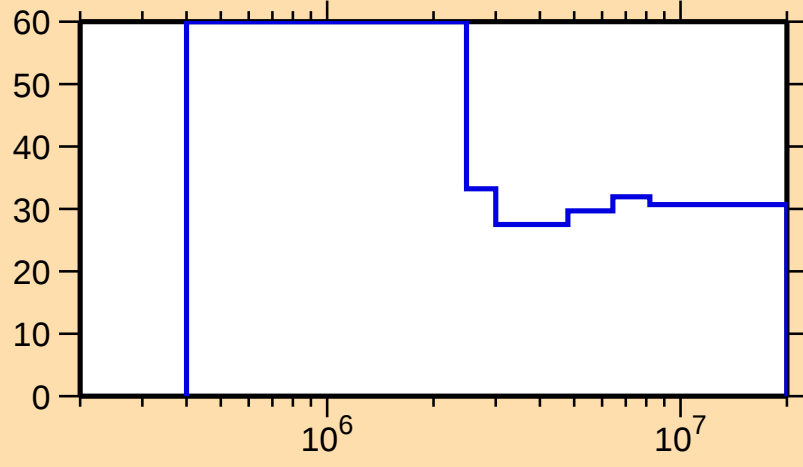
\Delta\sigma/\sigma vs. E for ^{172}\text{Lu}(n,n_1)
