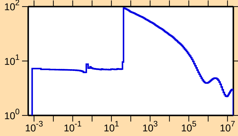
\sigma vs. E for ^{172}\text{Lu}(n,\text{el.})
