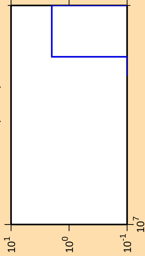
\Delta\sigma/\sigma vs. E for ^{172}\text{Lu}(\text{mt } 34)
