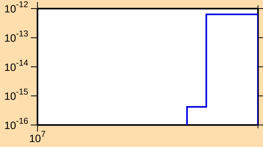
\sigma vs. E for ^{172}\text{Lu}(\text{mt } 34)
