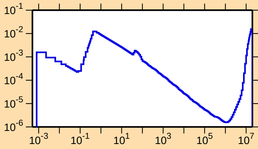
\sigma vs. E for ^{172}\text{Lu}(n,\alpha)
