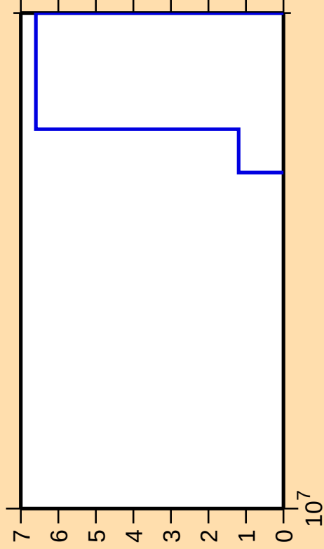
\Delta\sigma/\sigma vs. E for ^{172}\text{Lu}(\text{mt117})
