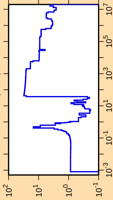
\Delta\sigma/\sigma vs. E for ^{172}\text{Lu}(n,\text{el.})
