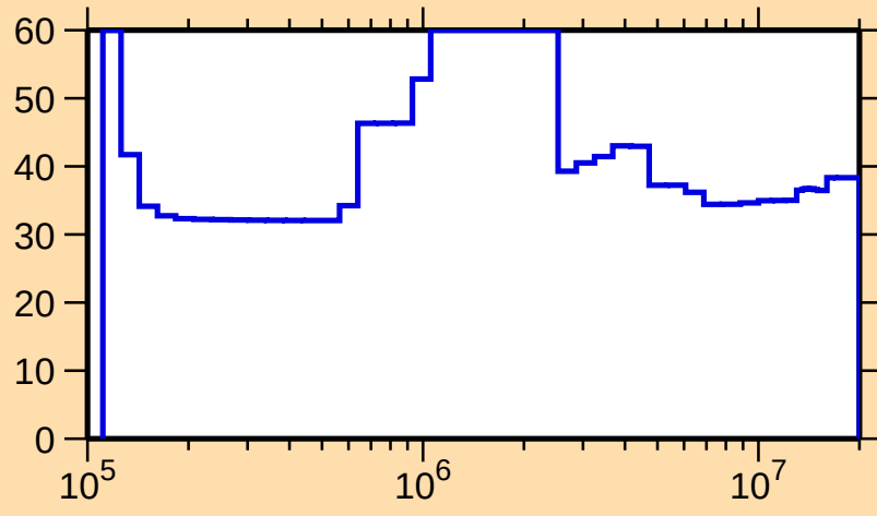
\Delta\sigma/\sigma vs. E for ^{173}\text{Lu}(n,n_1)
