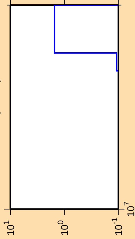
\Delta\sigma/\sigma vs. E for ^{173}\text{Lu} (mt 45)
