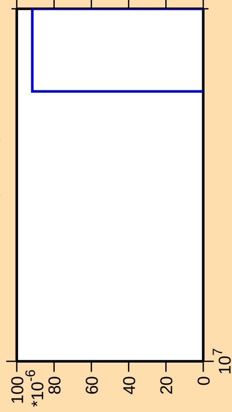
\Delta\sigma/\sigma vs. E for ^{173}\text{Lu} (mt 42)
