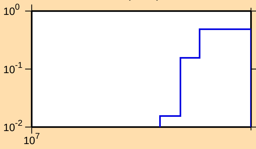
\sigma vs. E for ^{173}\text{Lu}(n,3n)
