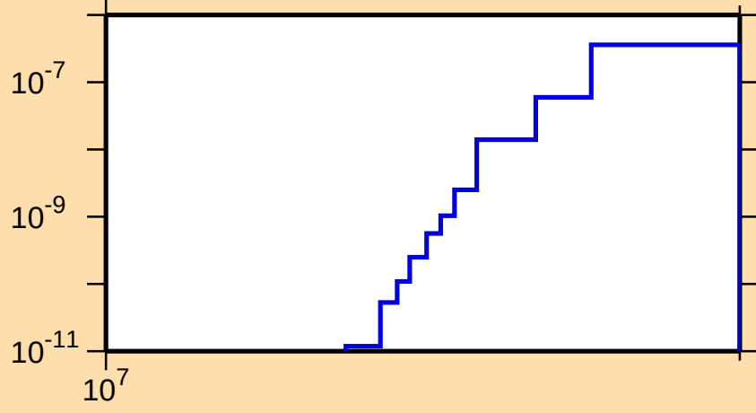
\sigma vs. E for ^{173}\text{Lu}(n,2n\alpha)
