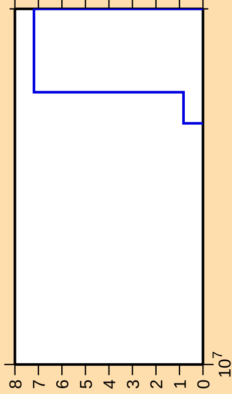
\Delta\sigma/\sigma vs. E for ^{173}\text{Lu}(\text{mt117})
