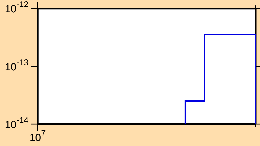
\sigma vs. E for ^{173}\text{Lu} (mt 45)
