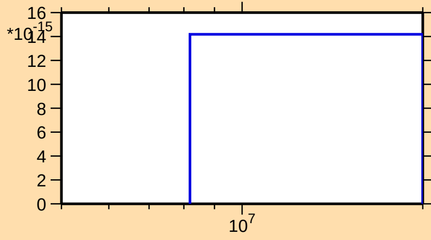
\sigma vs. E for ^{173}\text{Lu}(\text{mt117})
