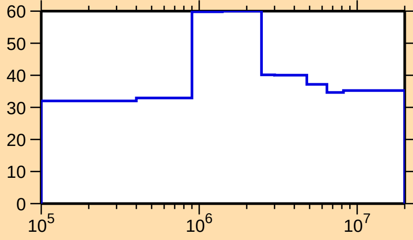
\Delta\sigma/\sigma vs. E for ^{173}\text{Lu}(n,n_1)
