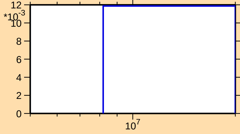
\sigma vs. E for ^{173}\text{Lu}(n,3n)
