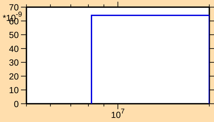
\sigma vs. E for ^{173}\text{Lu}(n,\text{nd})
