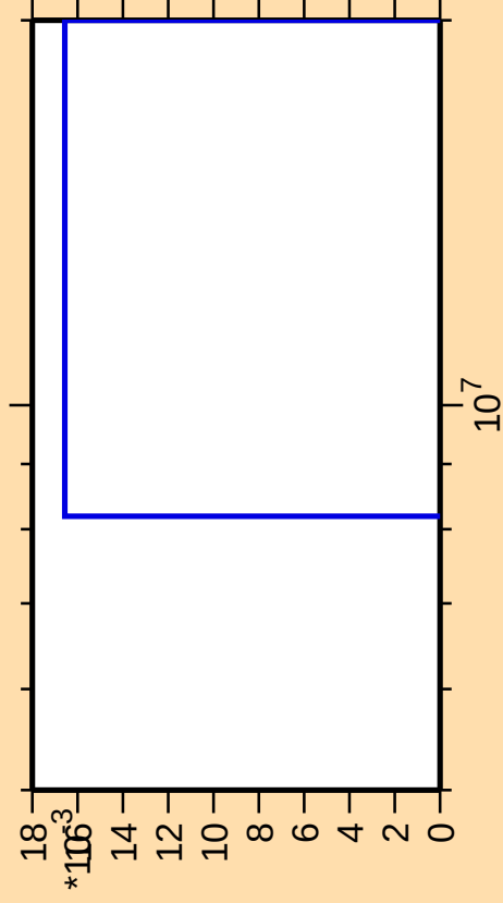
\Delta\sigma/\sigma vs. E for ^{173}\text{Lu} (mt 45)
