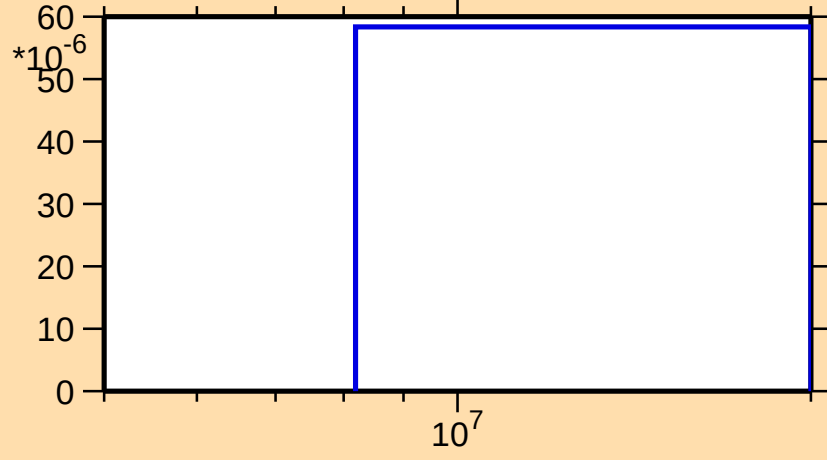
\sigma vs. E for ^{173}\text{Lu}(n,t)
