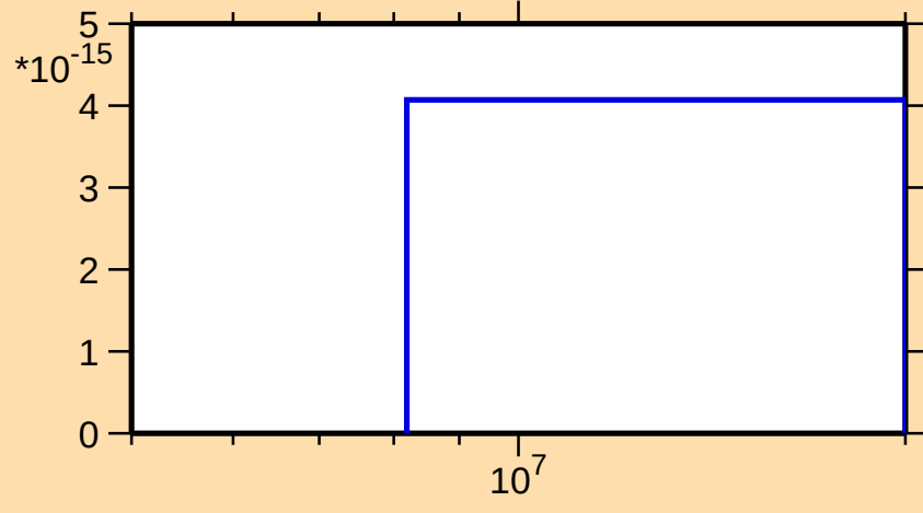
\sigma vs. E for ^{173}\text{Lu} (mt 45)
