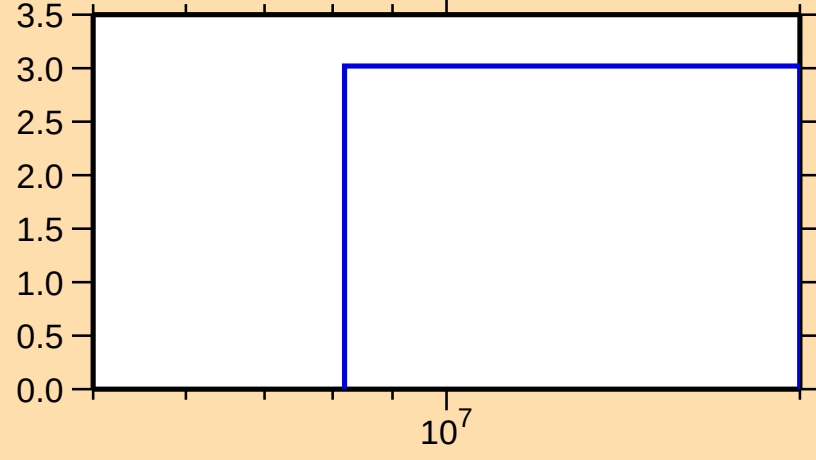
\Delta\sigma/\sigma vs. E for ^{173}\text{Lu}(n,\text{tot.})
