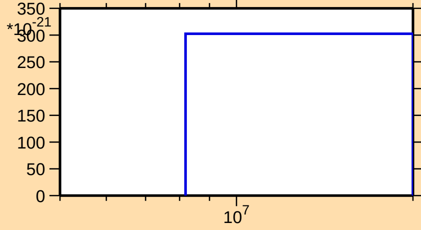
\sigma vs. E for ^{173}\text{Lu} (mt 42)
