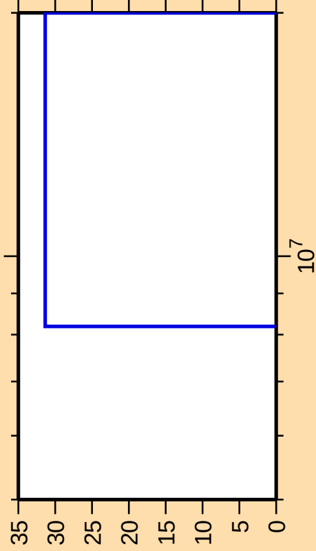
\Delta\sigma/\sigma vs. E for ^{173}\text{Lu}(n,3n)
