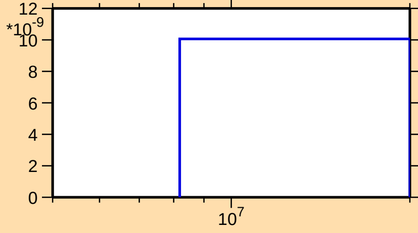
\sigma vs. E for ^{173}\text{Lu}(n,nt)
