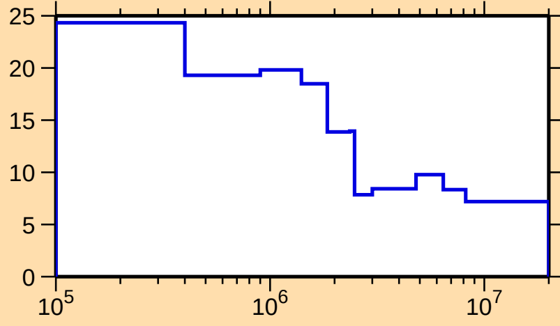
\Delta\sigma/\sigma vs. E for ^{173}\text{Lu}(n,\text{nonel.})
