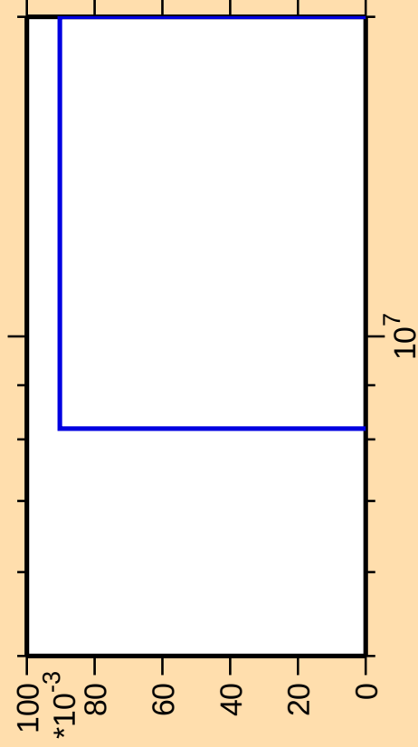
\Delta\sigma/\sigma vs. E for ^{173}\text{Lu}(\text{mt117})
