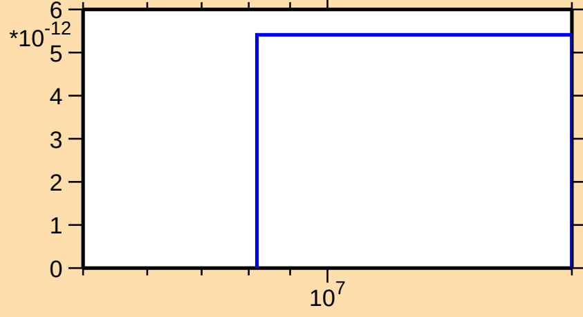
\sigma vs. E for ^{173}\text{Lu}(n,p\alpha)
