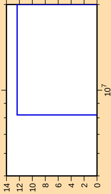
\Delta\sigma/\sigma vs. E for ^{173}\text{Lu}(n,2n)
