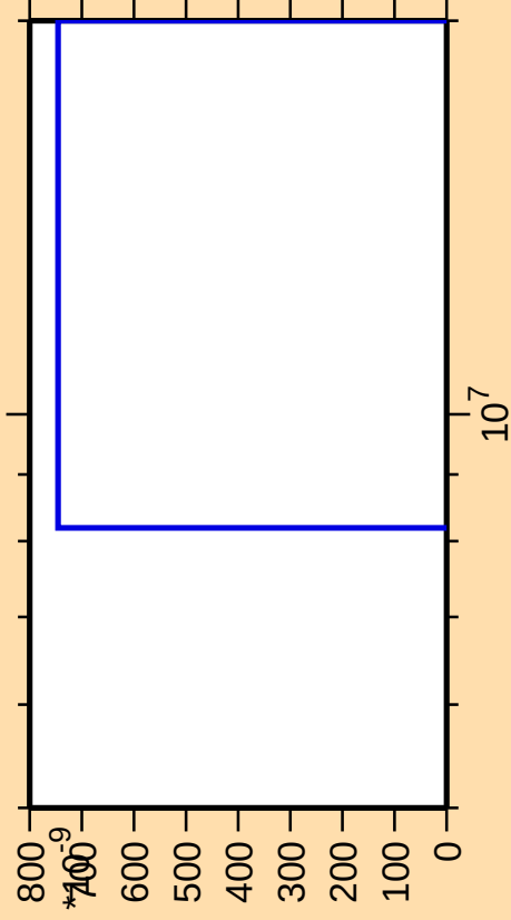
\Delta\sigma/\sigma vs. E for ^{173}\text{Lu} (mt 42)
