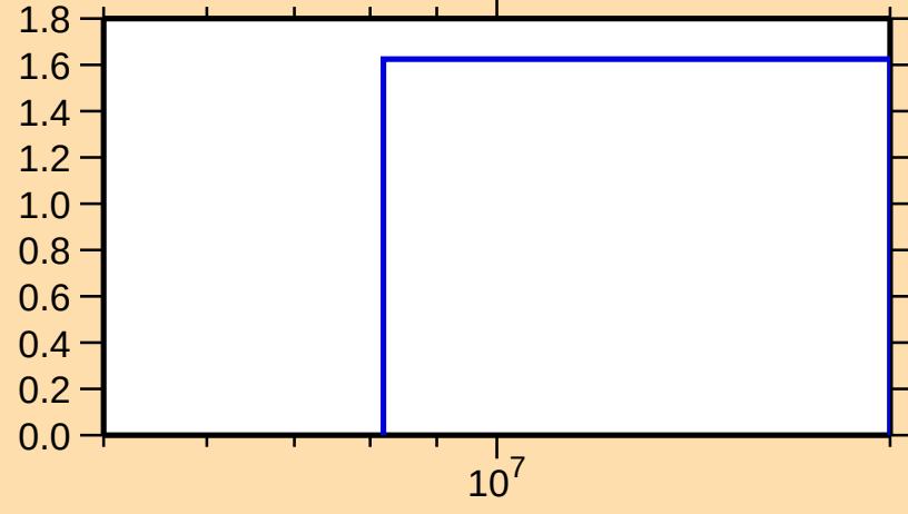
\sigma vs. E for ^{173}\text{Lu}(n,2n)
