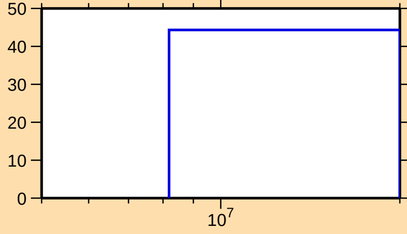
\Delta\sigma/\sigma vs. E for ^{173}\text{Lu}(n,\text{inel.})
