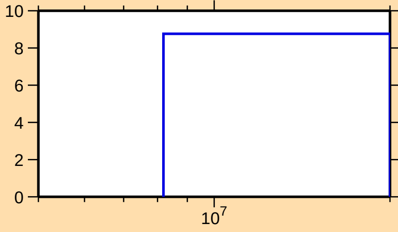
\Delta\sigma/\sigma vs. E for ^{173}\text{Lu}(n,\text{el.})
