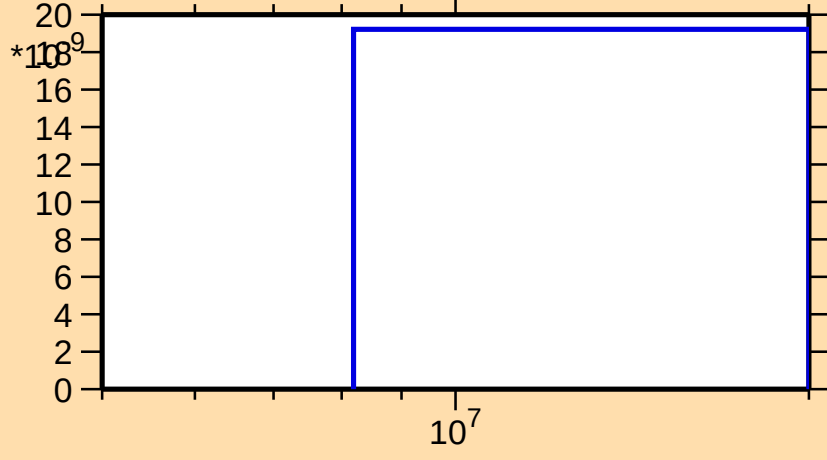
\sigma vs. E for ^{173}\text{Lu}(n,2np)
