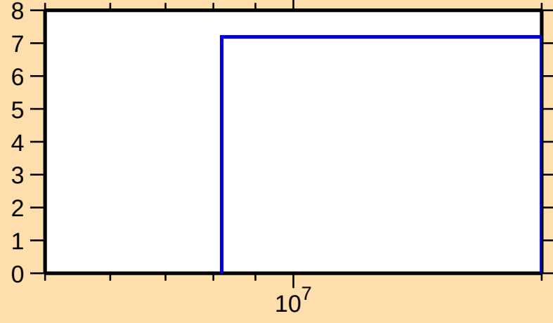
\Delta\sigma/\sigma vs. E for ^{173}\text{Lu}(n,\text{nonel.})
