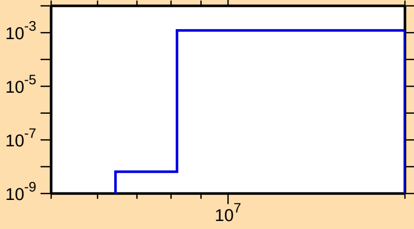
\sigma vs. E for ^{173}\text{Lu}(n,np)
