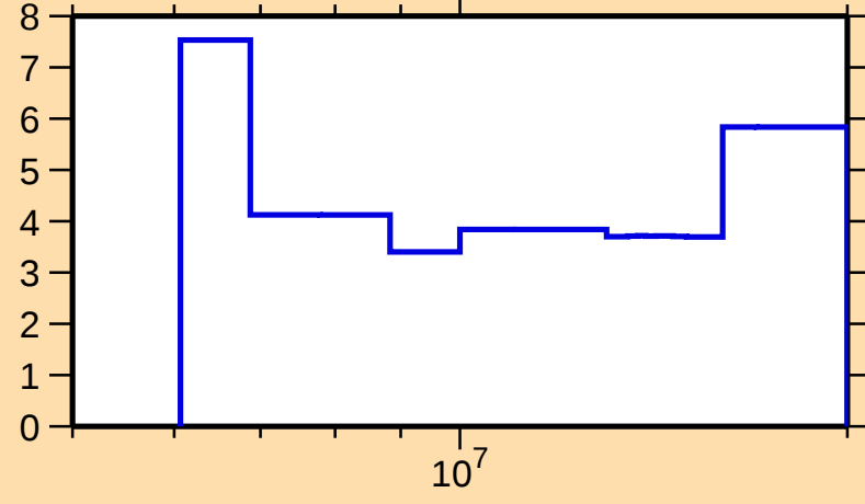
\Delta\sigma/\sigma vs. E for ^{174}\text{Lu}(n,\text{tot.})
