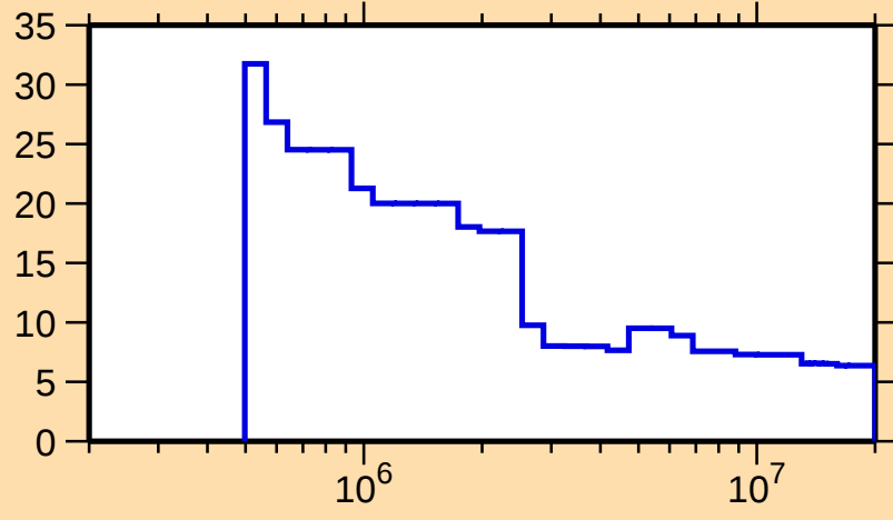
\Delta\sigma/\sigma vs. E for ^{174}\text{Lu}(n,\text{nonel.})
