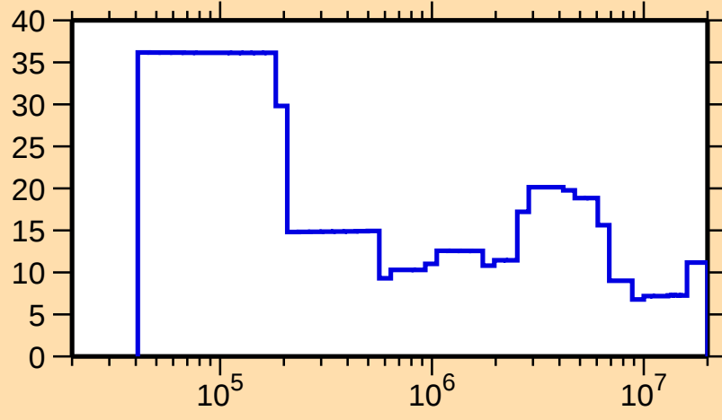
\Delta\sigma/\sigma vs. E for ^{174}\text{Lu}(n,\text{el.})
