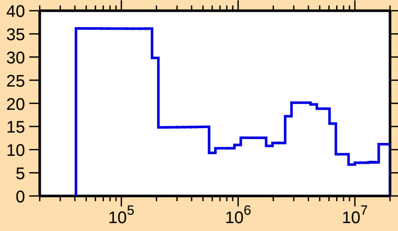
\Delta\sigma/\sigma vs. E for ^{174}\text{Lu}(\text{n,el.})
