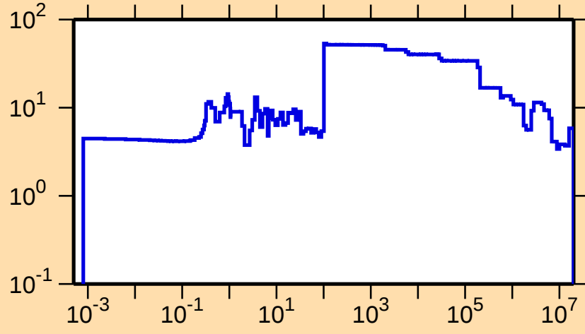
\Delta\sigma/\sigma vs. E for ^{174}\text{Lu}(n,\text{tot.})
