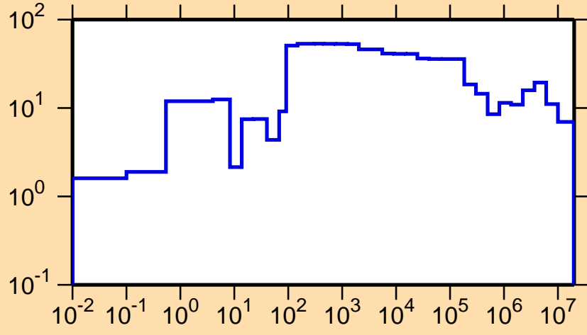
\Delta\sigma/\sigma vs. E for ^{174}\text{Lu}(n,el.)
