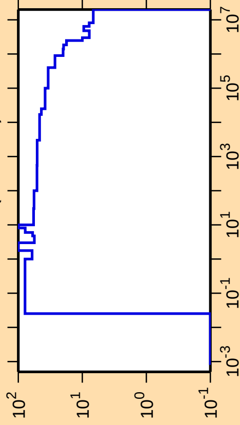
\Delta\sigma/\sigma vs. E for ^{174}\text{Lu}(n,\text{nonel.})
