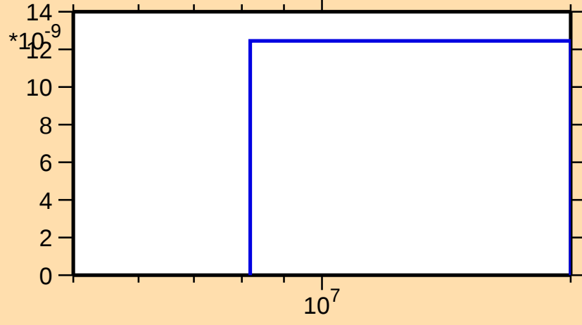
\sigma vs. E for ^{174}\text{Lu}(n,nt)
