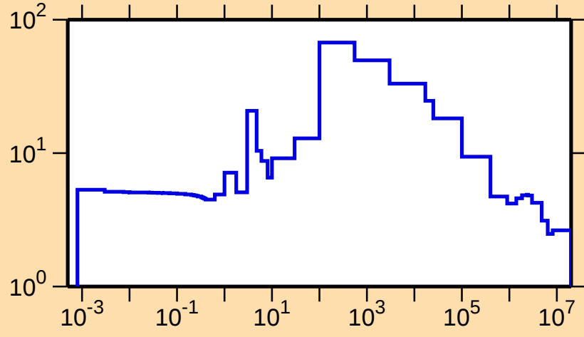
\sigma vs. E for ^{174}\text{Lu}(n,\text{el.})
