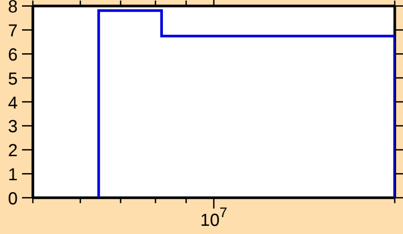
\Delta\sigma/\sigma vs. E for ^{174}\text{Lu}(n,\text{nonel.})
