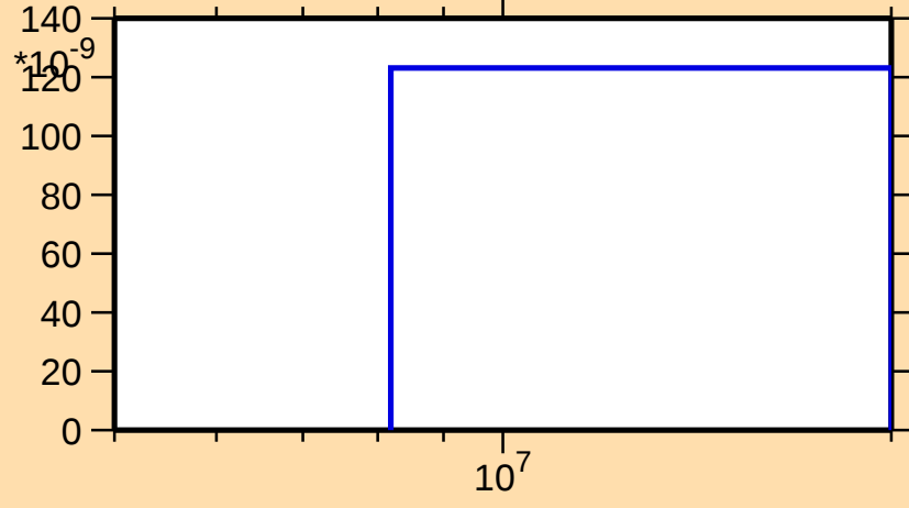
\sigma vs. E for ^{174}\text{Lu}(n,2np)
