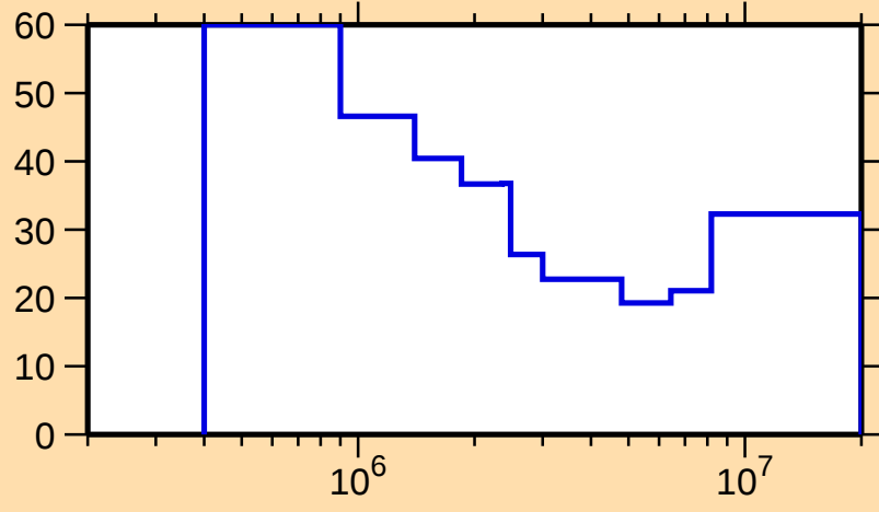
\Delta\sigma/\sigma vs. E for ^{174}\text{Lu}(n,n\text{cont.})
