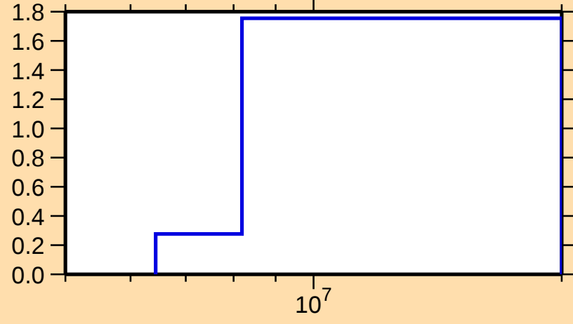
\sigma vs. E for ^{174}\text{Lu}(n,2n)
