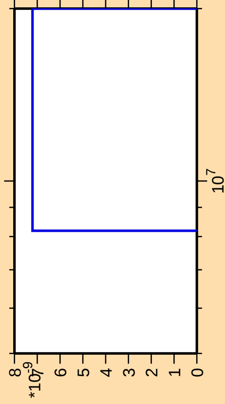
\Delta\sigma/\sigma vs. E for ^{174}\text{Lu}(\text{mt } 42)
