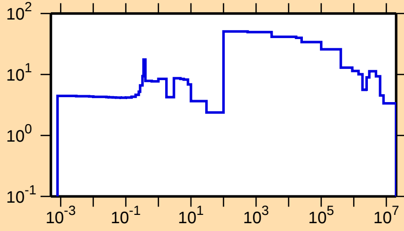
\Delta\sigma/\sigma vs. E for ^{174}\text{Lu}(\text{n,tot.})
