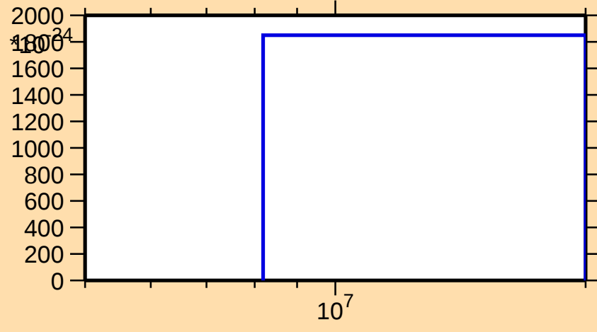
\sigma vs. E for ^{174}\text{Lu}(\text{mt } 42)
