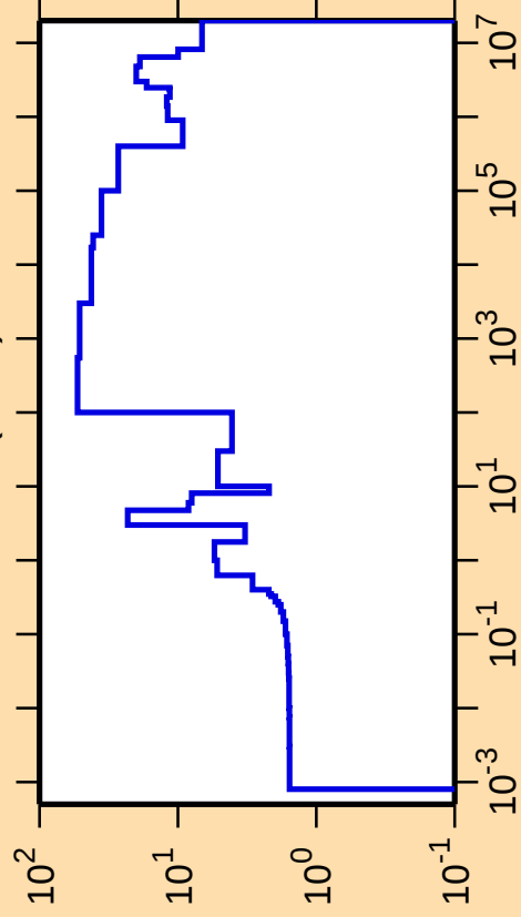
\Delta\sigma/\sigma vs. E for ^{174}\text{Lu}(\text{n,el.})
