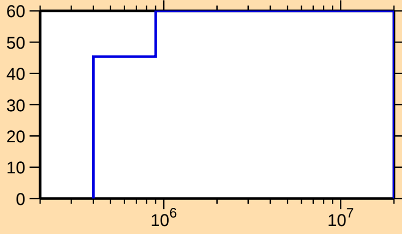
\Delta\sigma/\sigma vs. E for ^{174}\text{Lu}(n,n_1)
