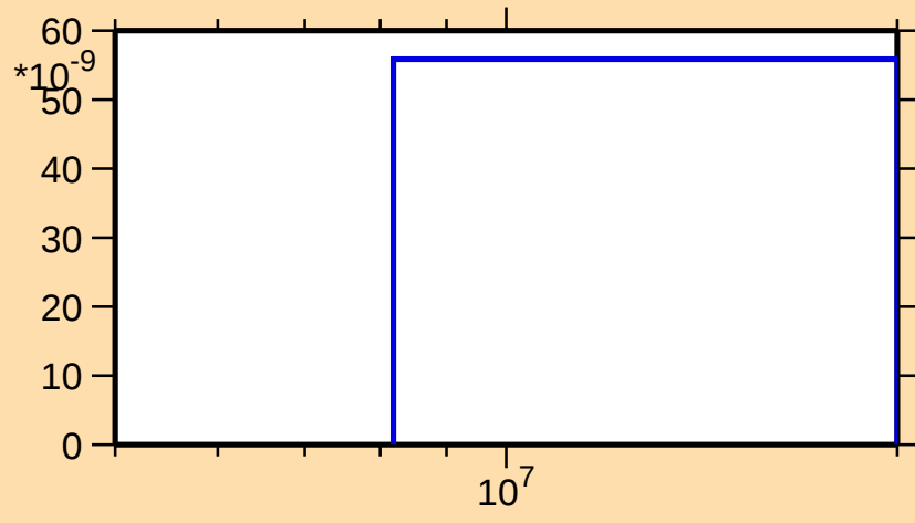
\sigma vs. E for ^{174}\text{Lu}(n,2n\alpha)
