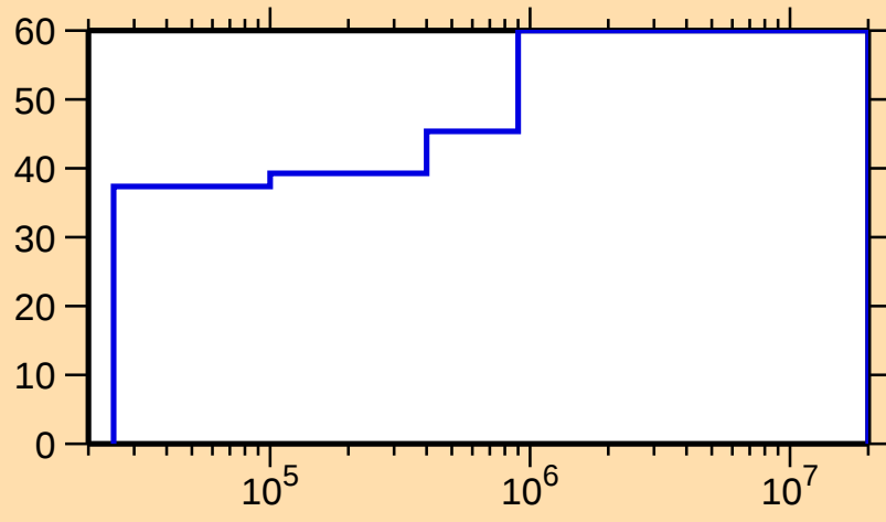
\Delta\sigma/\sigma vs. E for ^{174}\text{Lu}(n,n_1)
