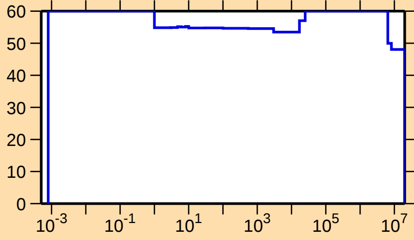
\Delta\sigma/\sigma vs. E for ^{174}\text{Lu}(n,p)
