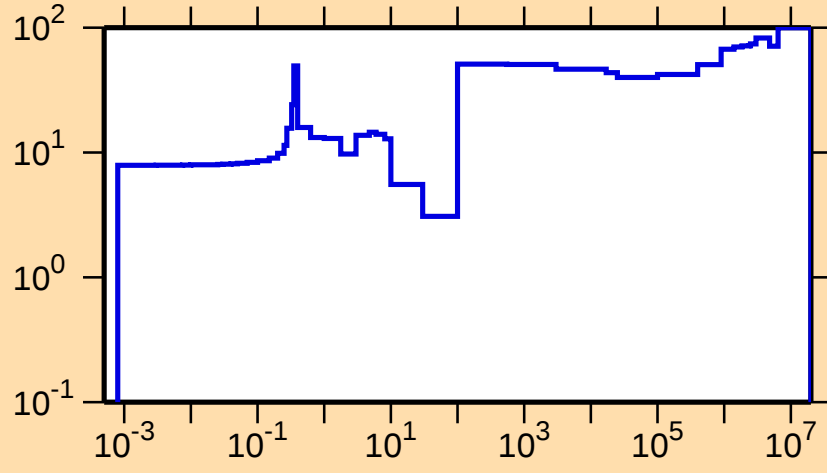
\Delta\sigma/\sigma vs. E for ^{174}\text{Lu}(n,\gamma)
