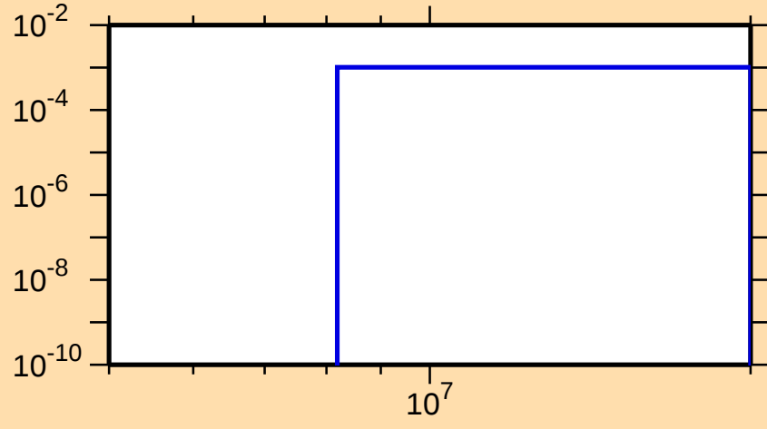
\sigma vs. E for ^{174}\text{Lu}(n,np)
