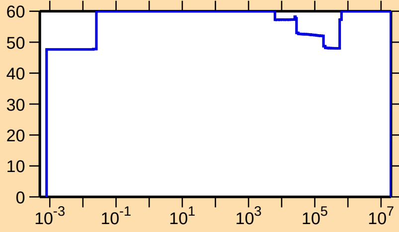
\Delta\sigma/\sigma vs. E for ^{174}\text{Lu}(n,p)
