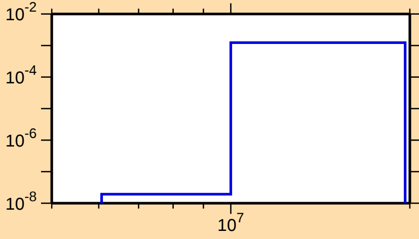
\sigma vs. E for ^{174}\text{Lu}(n,np)
