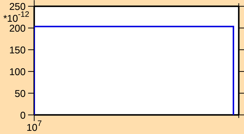
\sigma vs. E for ^{174}\text{Lu}(n,\text{He3})
