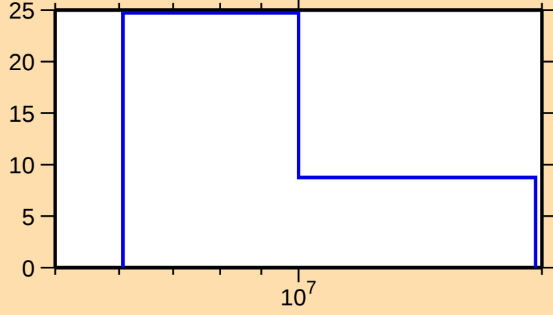
\Delta\sigma/\sigma vs. E for ^{174}\text{Lu}(n,2n)
