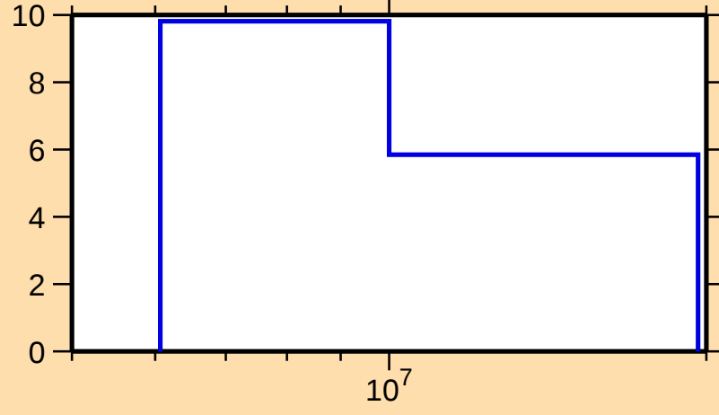
\Delta\sigma/\sigma vs. E for ^{174}\text{Lu}(n,\text{el.})
