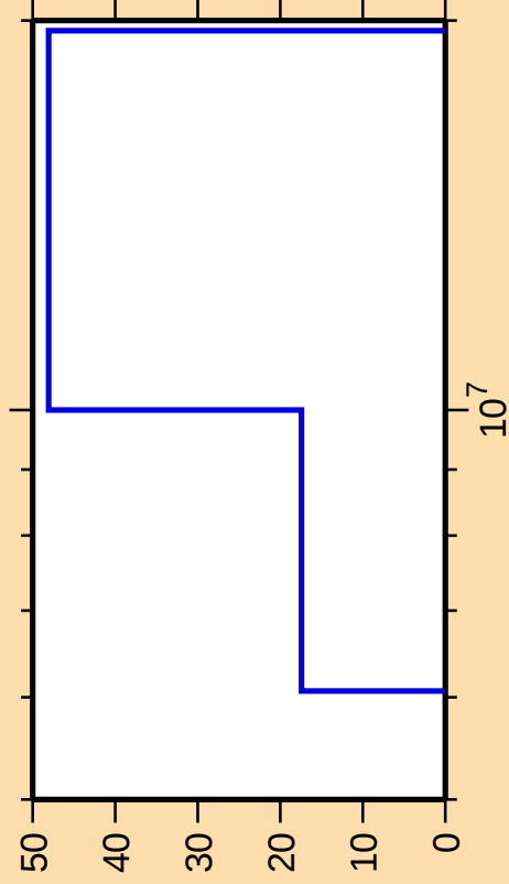
\Delta\sigma/\sigma vs. E for ^{174}\text{Lu}(n,n\text{cont.})
