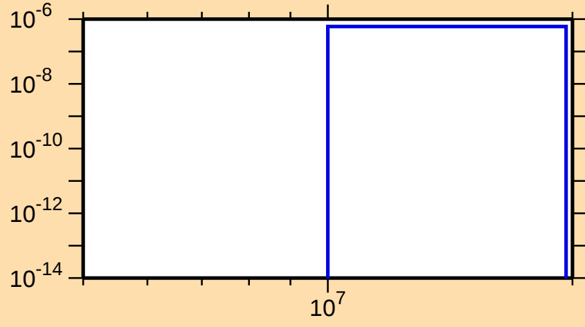
\sigma vs. E for ^{174}\text{Lu}(n,\text{nd})
