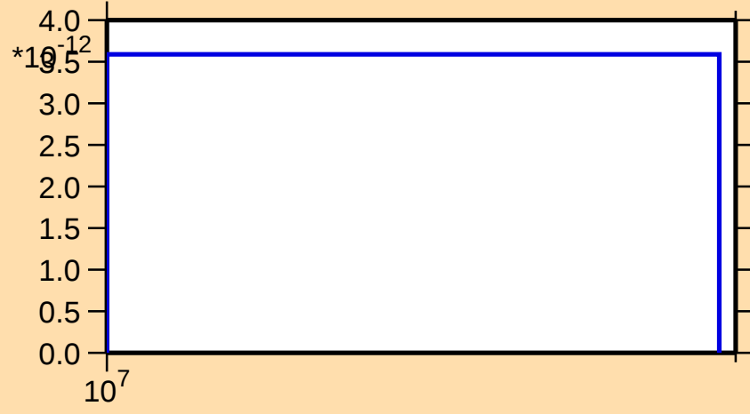
\sigma vs. E for ^{174}\text{Lu}(n,p\alpha)
