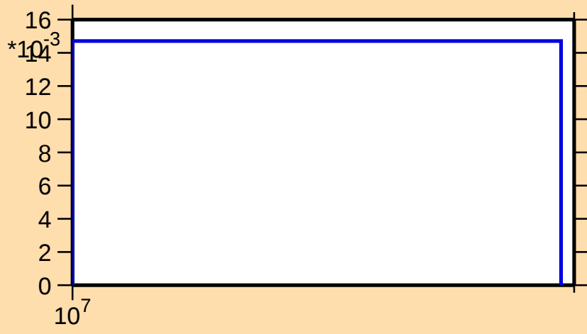
\sigma vs. E for ^{174}\text{Lu}(n,3n)
