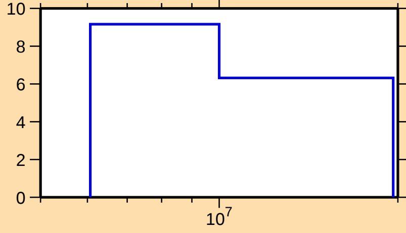
\Delta\sigma/\sigma vs. E for ^{174}\text{Lu}(n,\text{nonel.})
