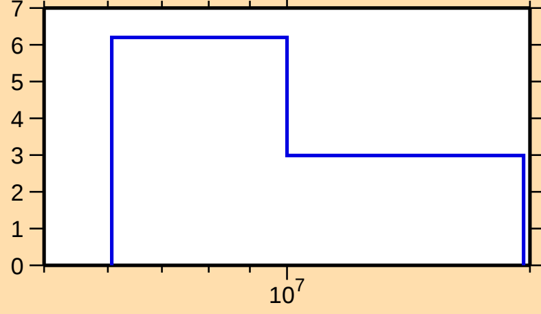
\Delta\sigma/\sigma vs. E for ^{174}\text{Lu}(n,\text{tot.})
