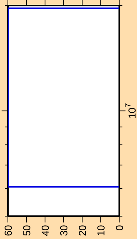
\Delta\sigma/\sigma vs. E for ^{174}\text{Lu}(n,p)
