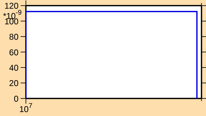
\sigma vs. E for ^{174}\text{Lu}(n,2np)
