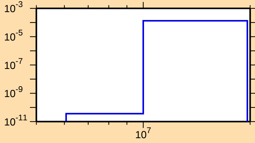
\sigma vs. E for ^{174}\text{Lu}(n,t)
