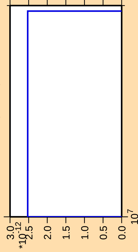
\Delta\sigma/\sigma vs. E for ^{174}\text{Lu} (mt 42)
