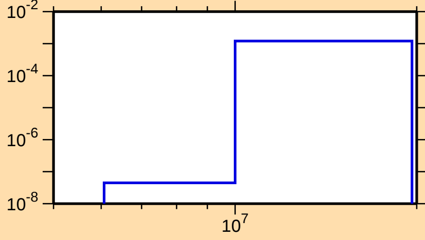
\sigma vs. E for ^{174}\text{Lu}(n,d)
