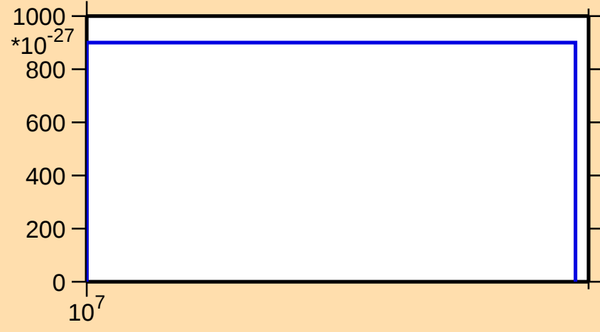
\sigma vs. E for ^{174}\text{Lu} (mt 42)
