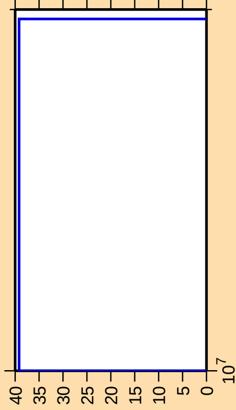
\Delta\sigma/\sigma vs. E for ^{174}\text{Lu}(n,3n)
