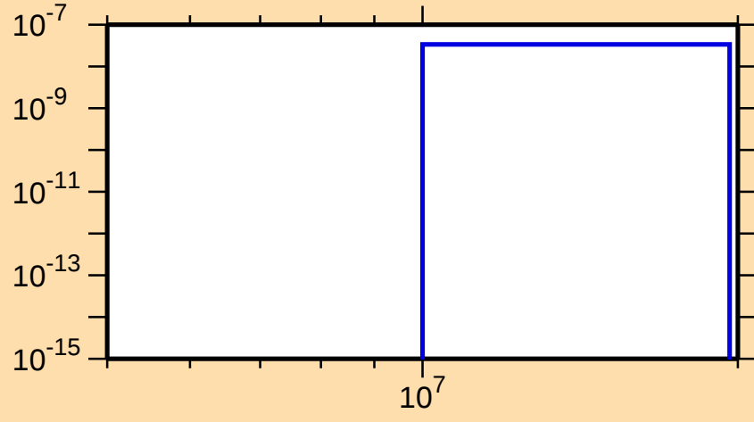
\sigma vs. E for ^{174}\text{Lu}(n,2n\alpha)
