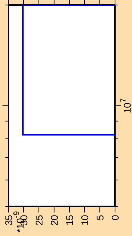
\Delta\sigma/\sigma vs. E for ^{174}\text{Lu} (mt 42)
