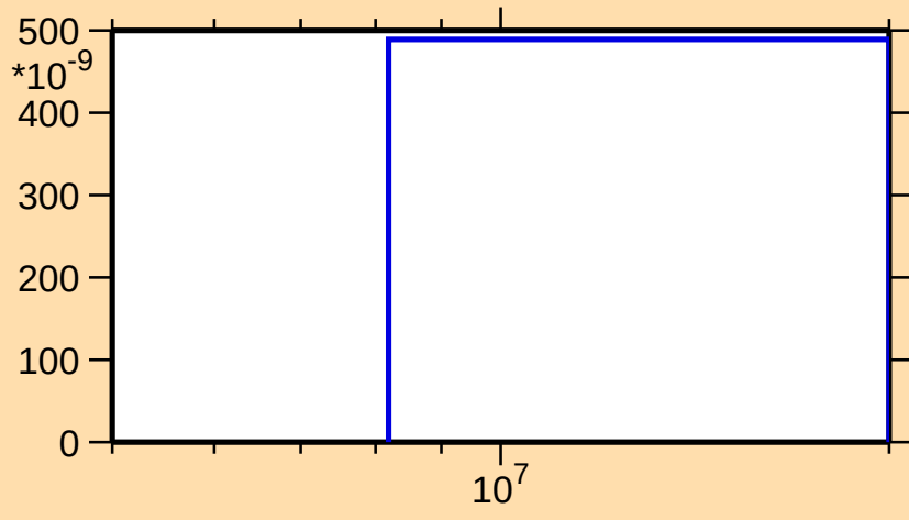
\sigma vs. E for ^{174}\text{Lu}(n,\text{nd})
